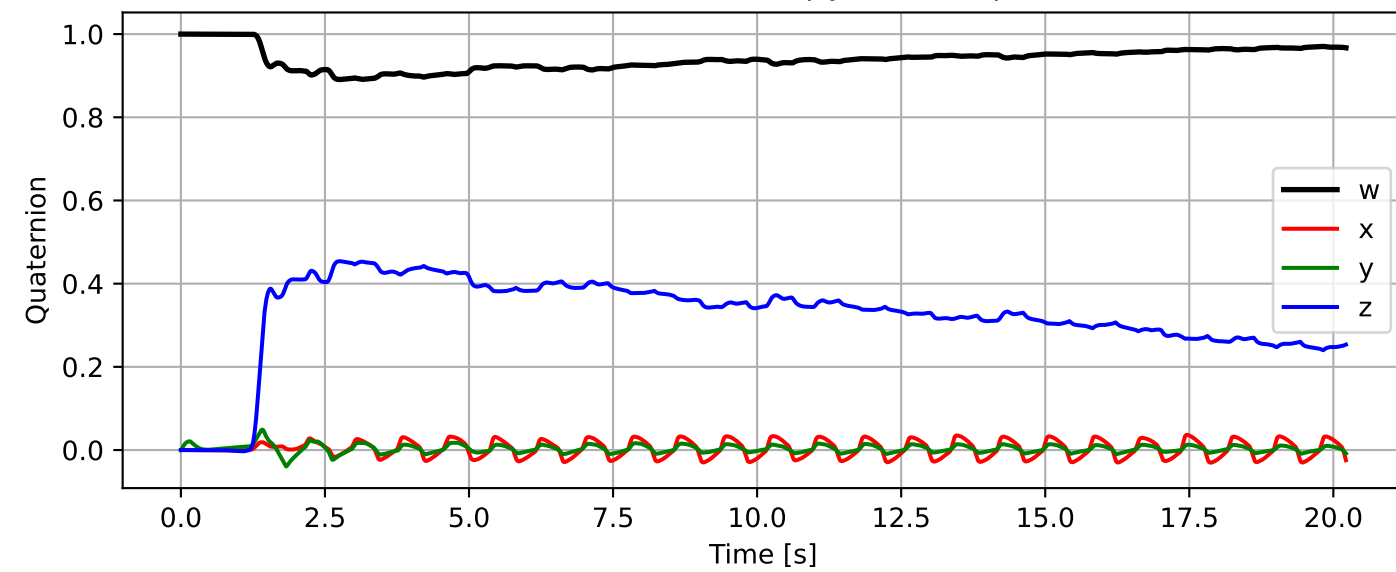
Base Orientation (Quaternion)
