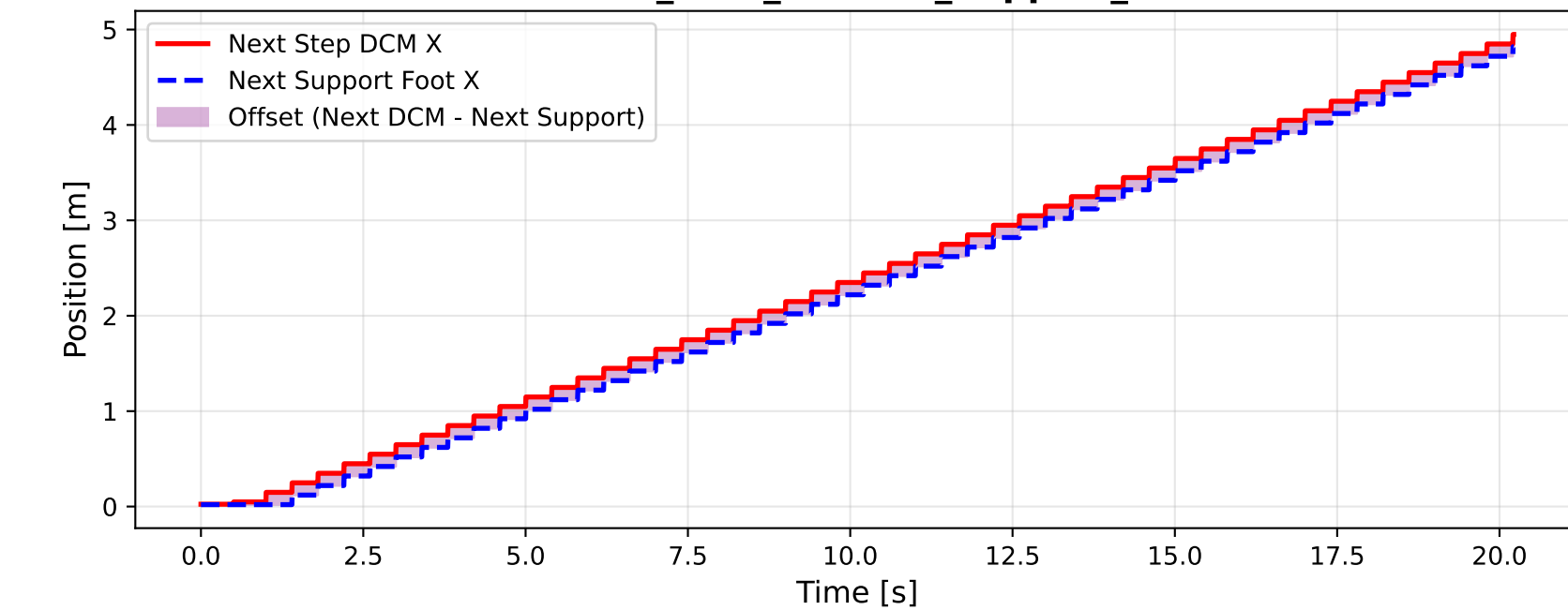
Desired DCM Offset Components (X)
