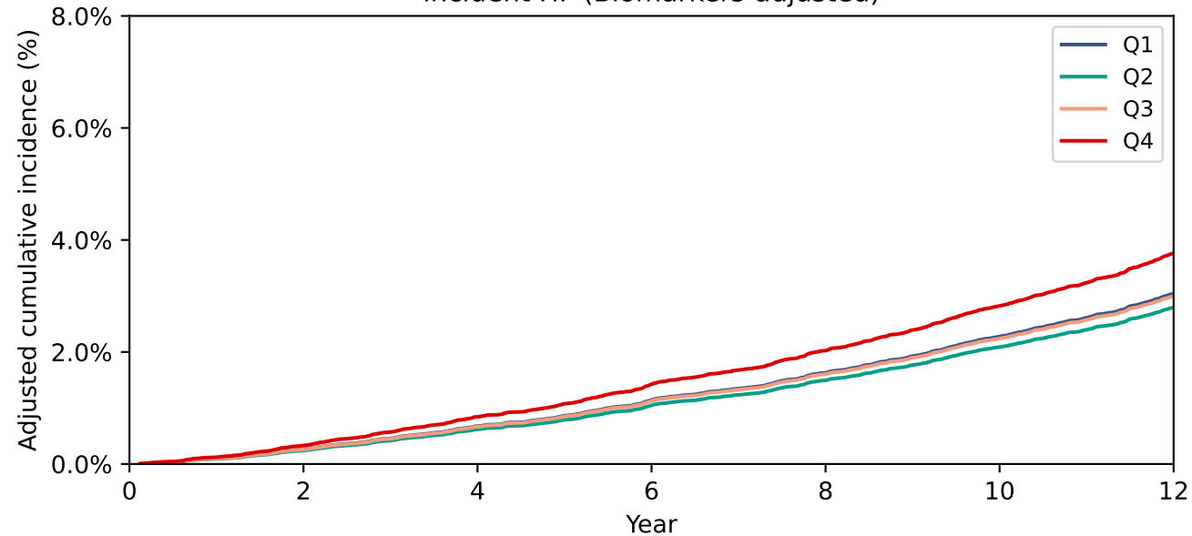
Incident HF (Biomarkers-adjusted)
