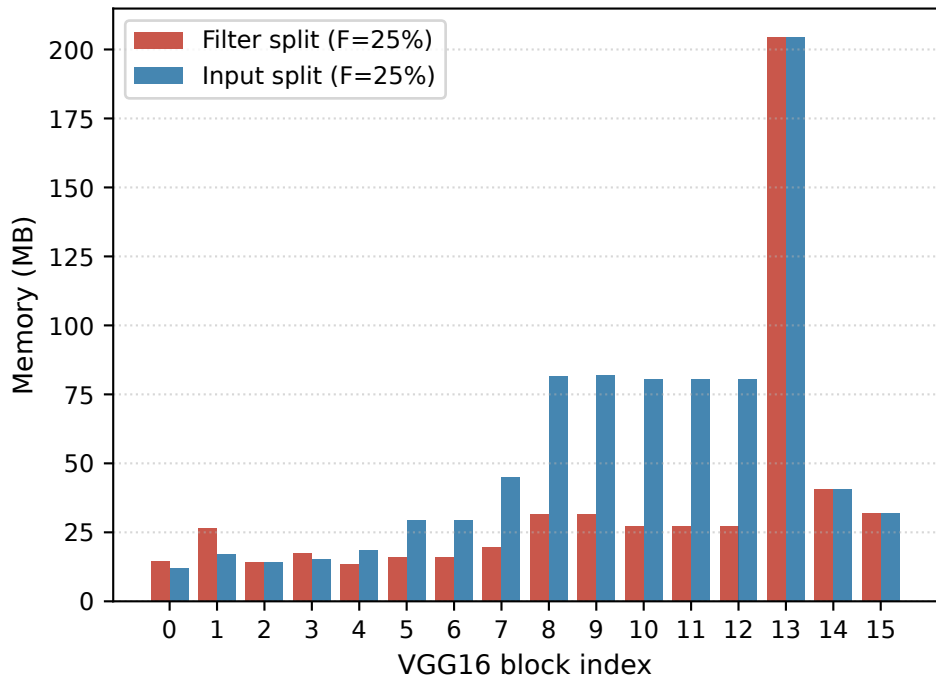
Memory consumption: filter vs input partitioning (F=25%)
