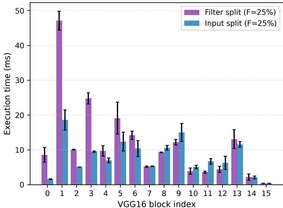
Execution time: filter vs input partitioning (F=25%)
