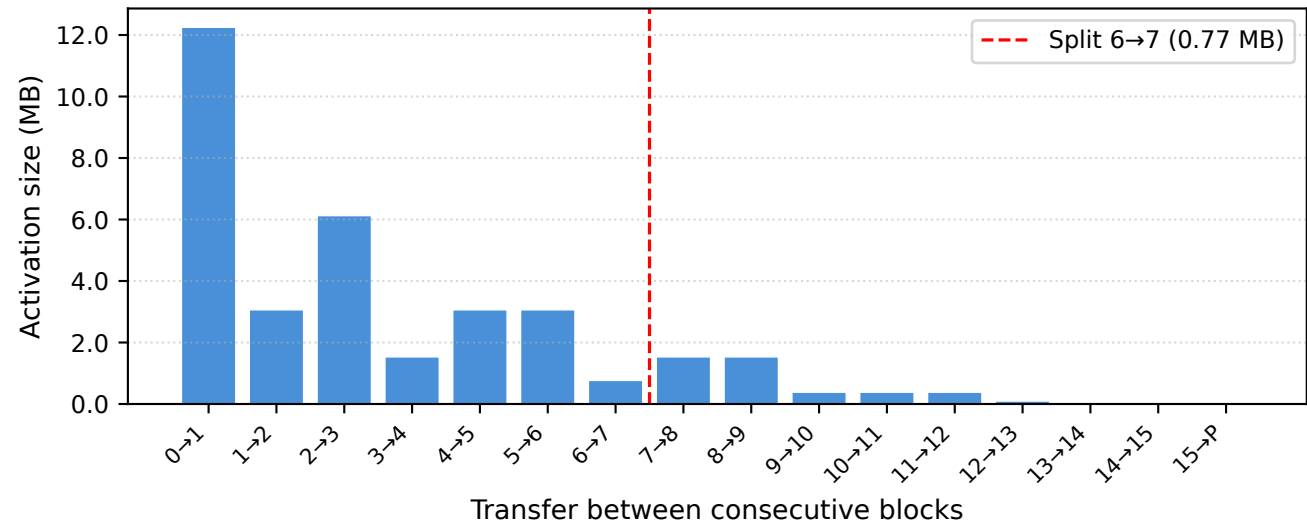
Intermediate feature map sizes transferred between VGG16 blocks
