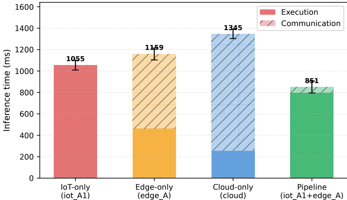
End-to-end VGG16 inference time by deployment strategy
