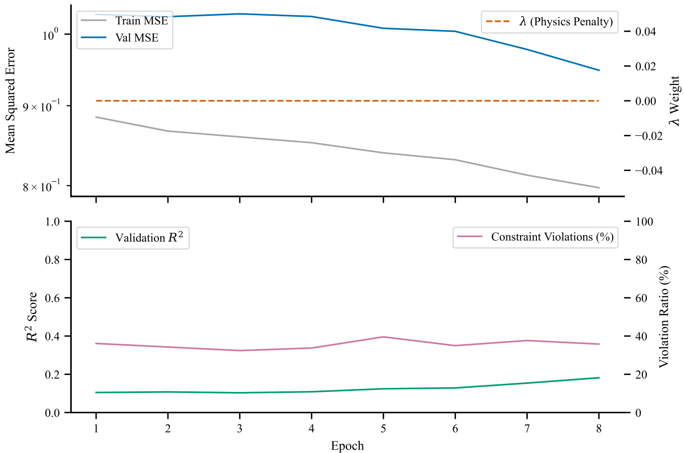
Model Convergence vs. Physics Constraint Annealing
