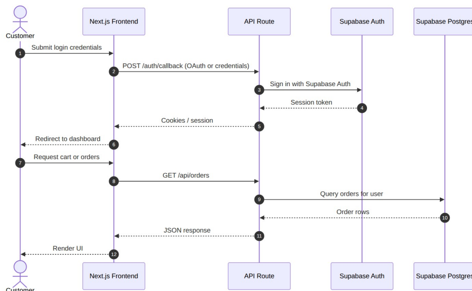
Figure 3.1 — Login / session sequence (from auth callback route and lib code).
