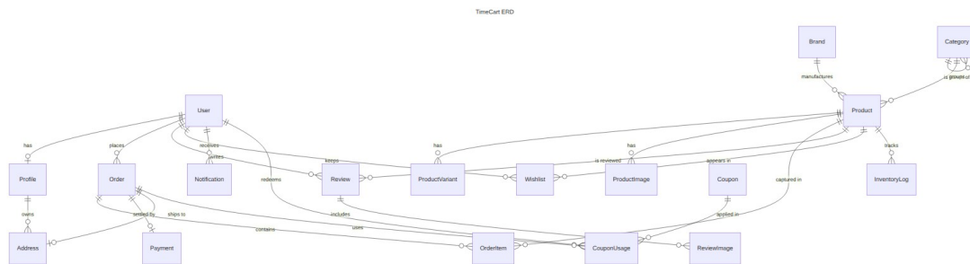
Figure 2.1 — Entity Relationship Diagram (generated from prisma/schema.prisma relations).
