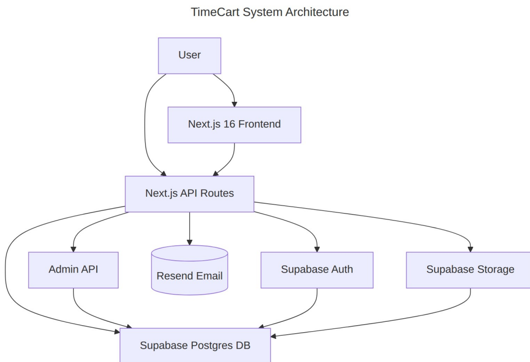
Figure 1.1 — System architecture (from source structure and configuration).
