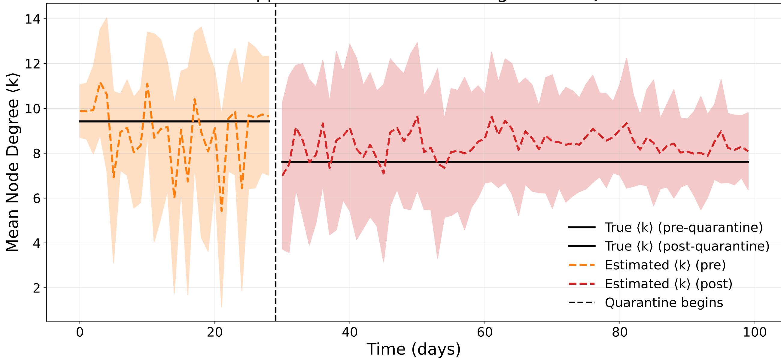
Mean Field Approximation Estimated Degree with Quarantine
