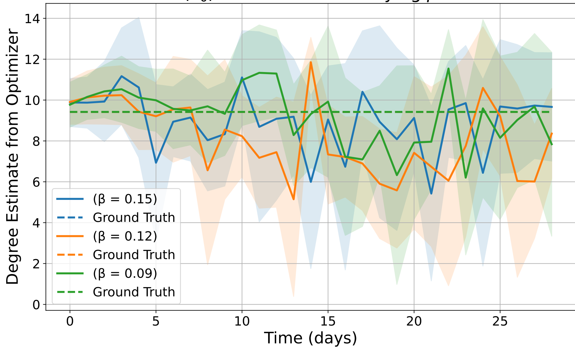
\langle k_0 \rangle Estimates with Varying \beta
