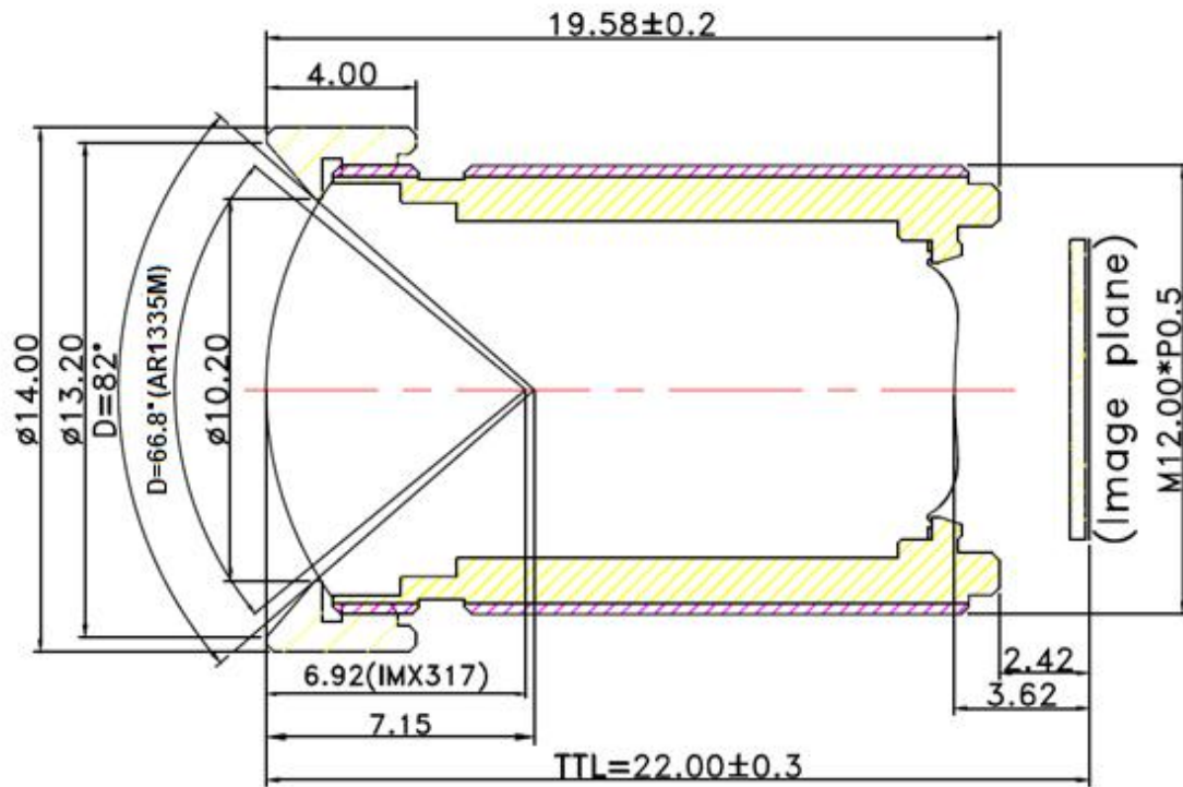
Figure 1: Lens Mechanical Dimensions
