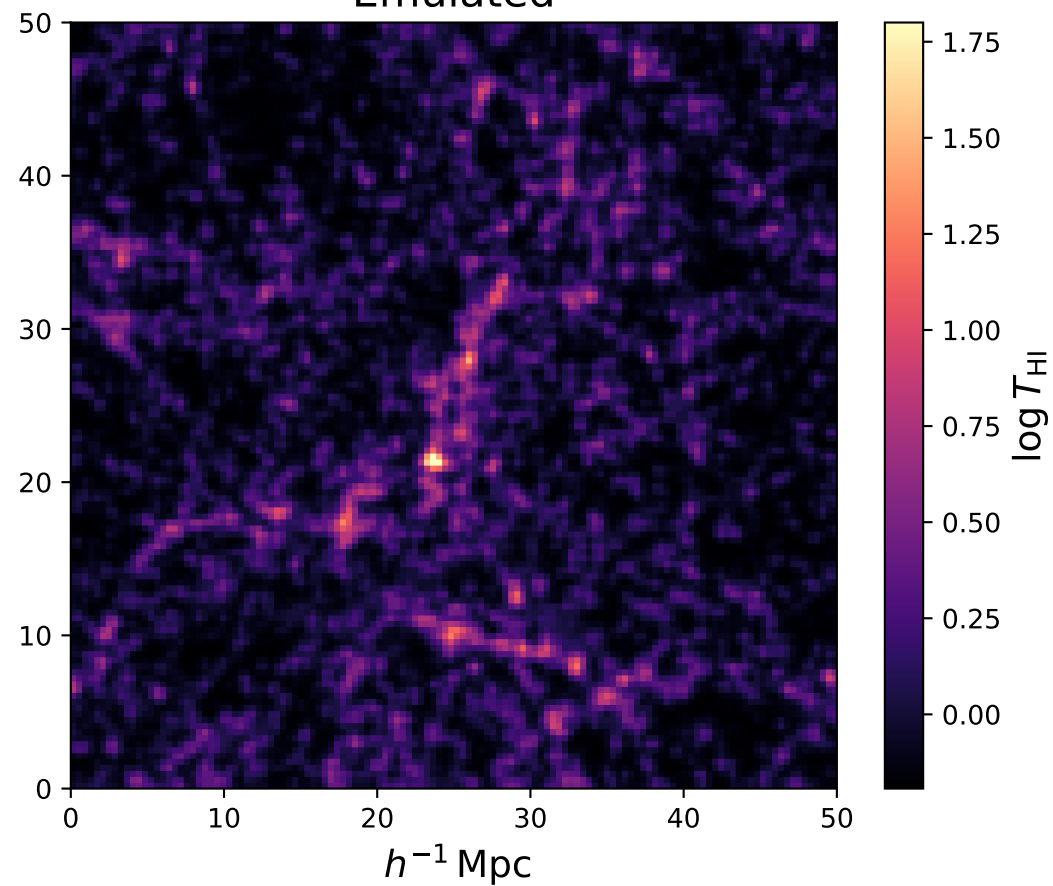
\log T_{\text{HI}} distribution
