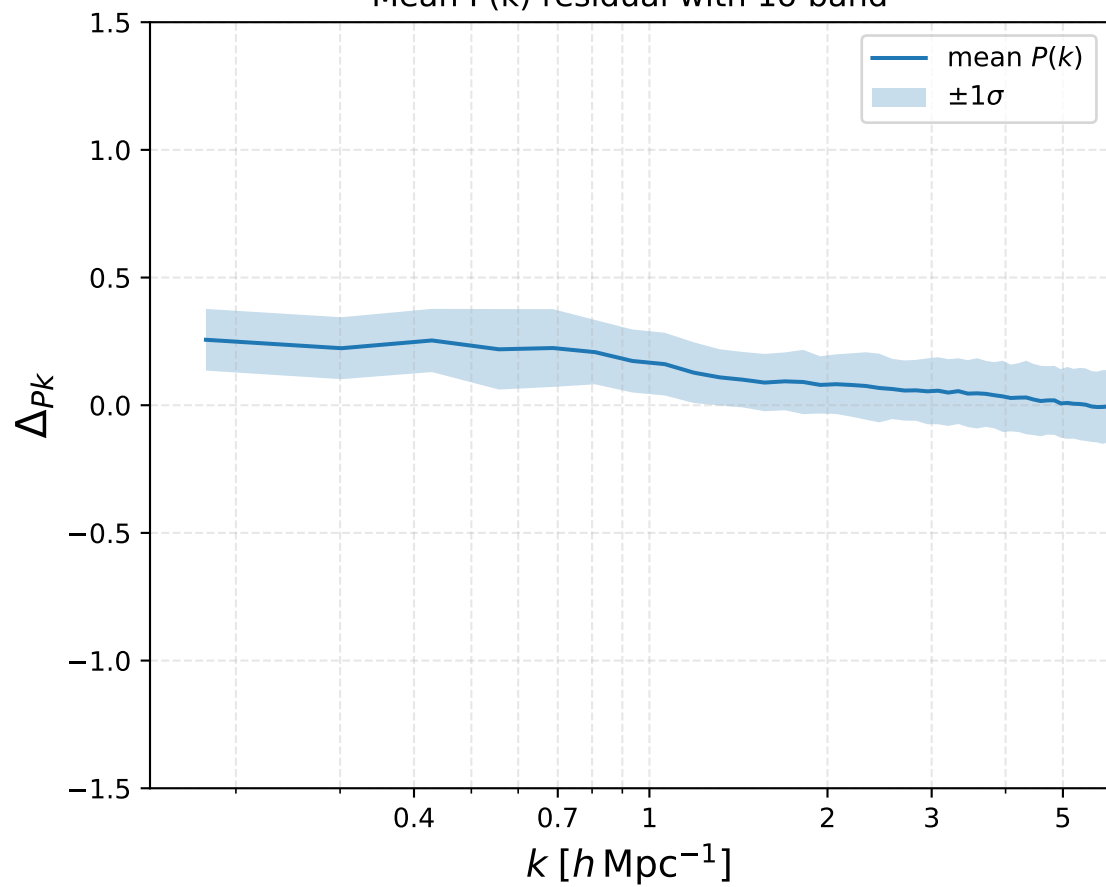
Mean P(k) residual with 1\sigma band
