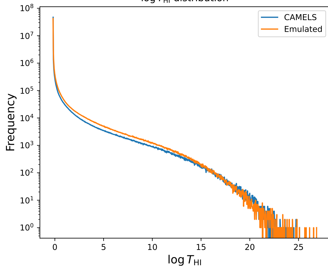
\log T_{\text{HI}} distribution
