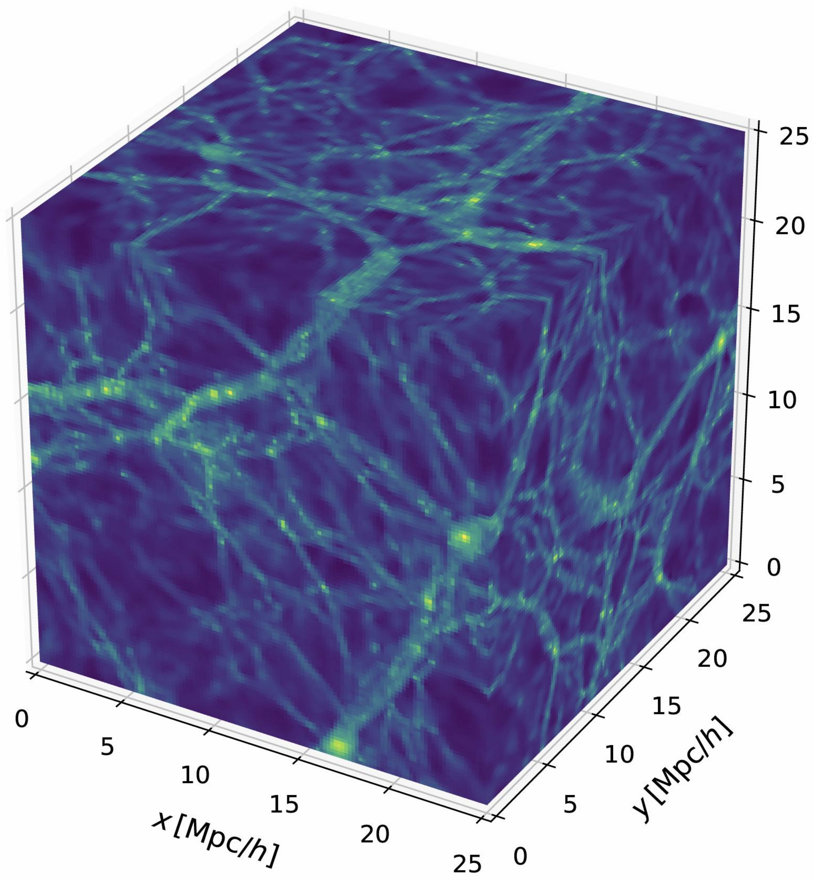
Ground truth
