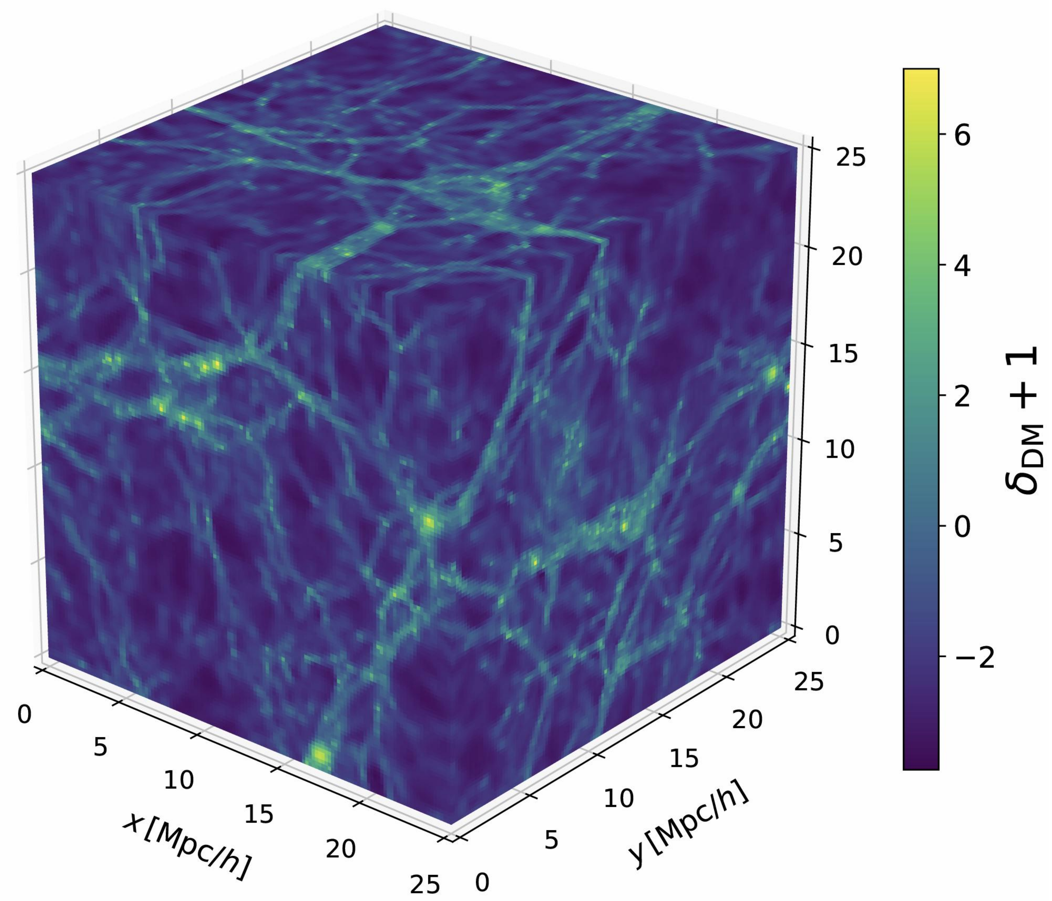
Generated sample 1
