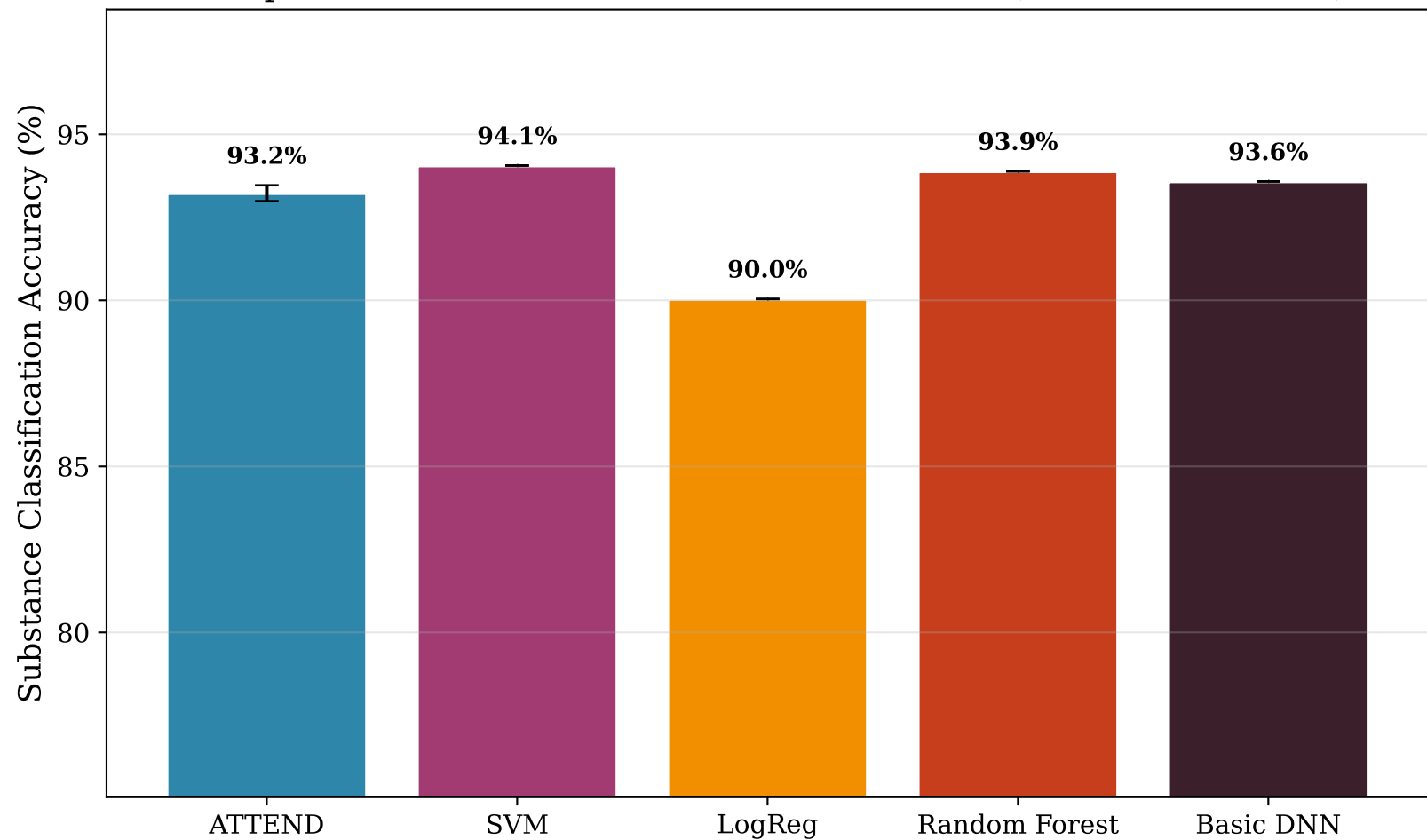
Comparison of Models: Substance Classification (Combined Dataset)
