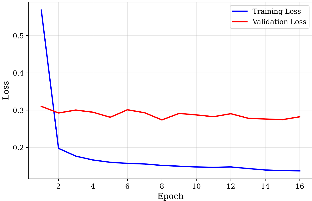
ATTEND Training and Validation Loss (Combined Dataset)
