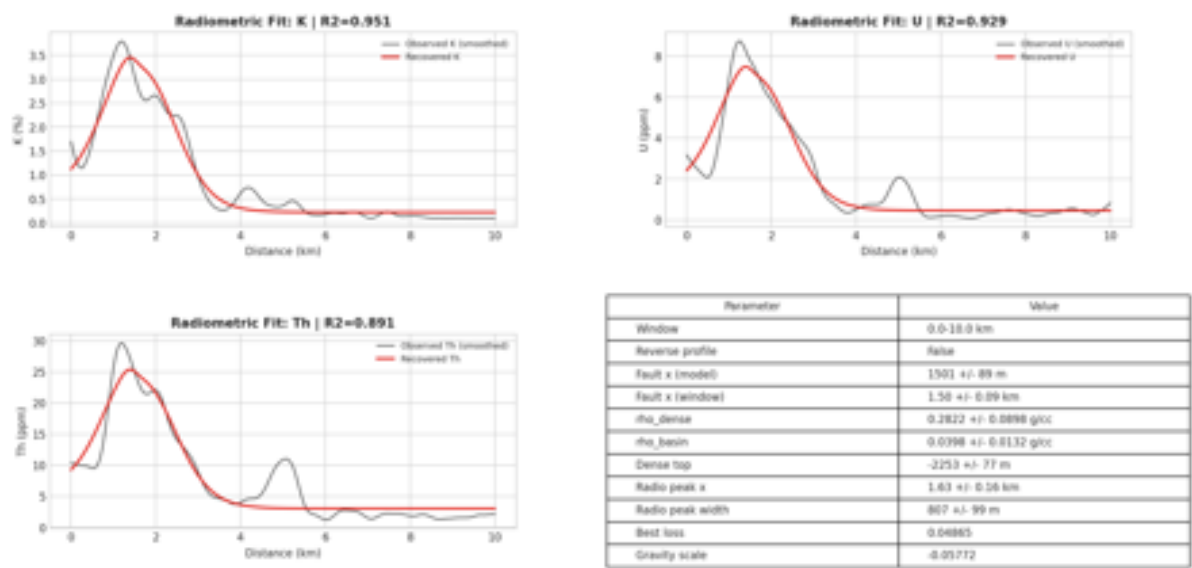
Figure 10: Stage 2 K, U, and Th fits for the best 10 km real-data inversion.
