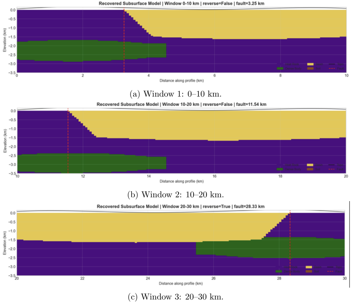
Figure 14: Individual recovered geological/subsurface profiles for all three Stage 3 windows.
