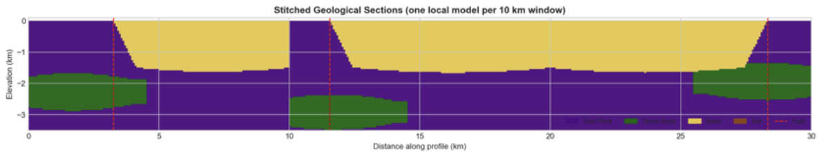
Figure 13: Stage 3 stitched geological section across the 30 km profile. Each 10 km section is independently inverted and then placed in global distance coordinates.
