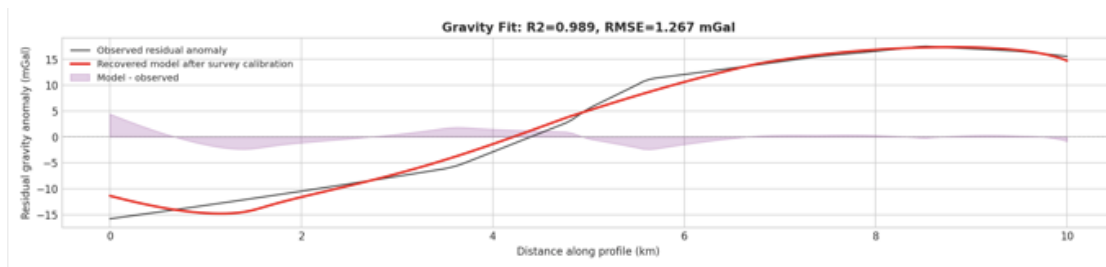
Figure 9: Stage 2 gravity fit for the selected 10 km real-data window. The calibrated gravity response reaches R^2 = 0.989 and RMSE = 1.267 mGal.
