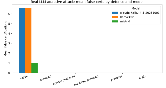
Figure 3: Real-LLM adaptive attack: mean false certifications by defense and model. Firewall arms suppress false discoveries across every model tested.
