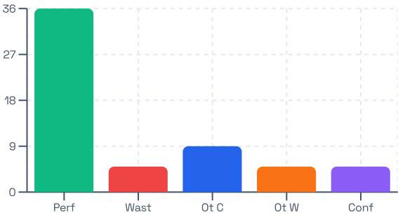
ATTEMPT PROFILE
