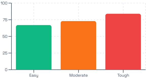
DIFFICULTY ACCURACY
