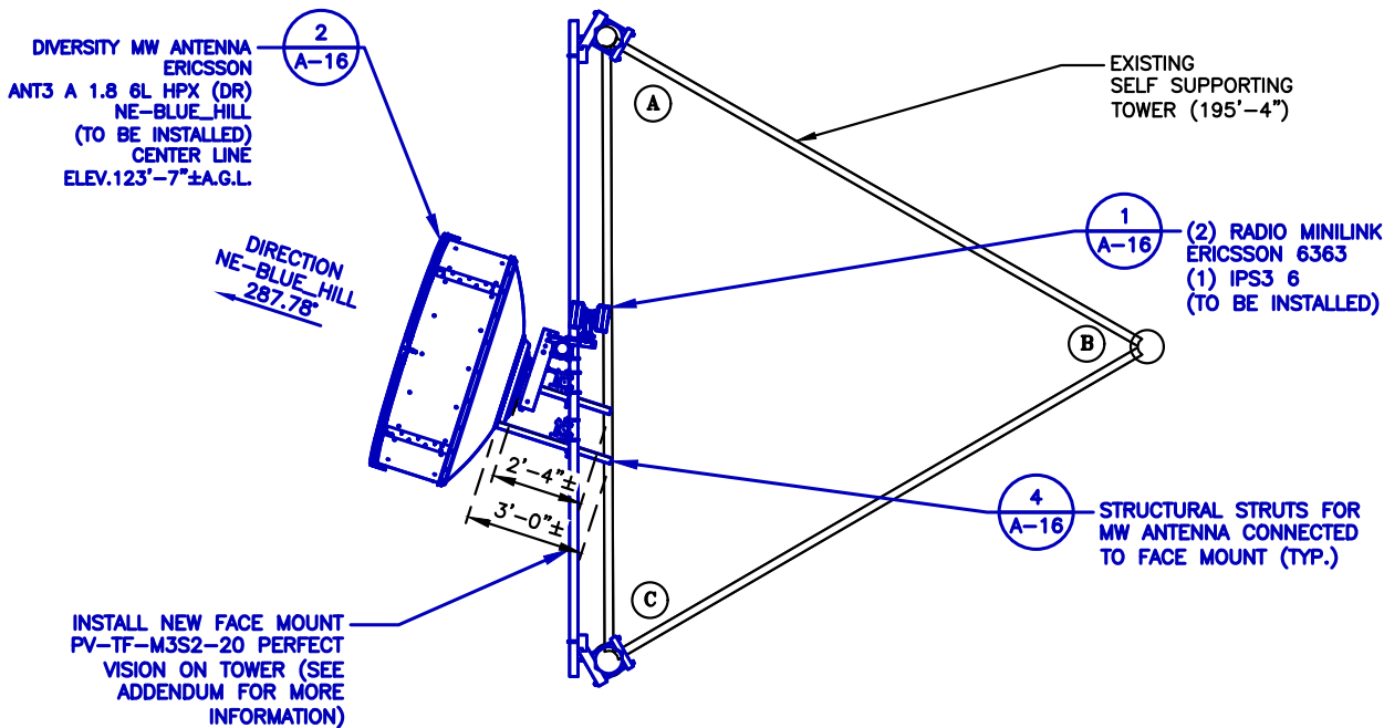
PROPOSED MW ANTENNA PLAN
