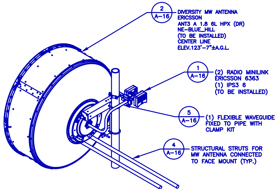
PROPOSED DIVERSITY MW ANTENNA ANT3 A 1.8 6L HPX (DR) DETAIL
