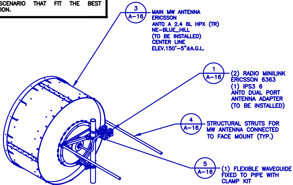
PROPOSED MAIN MW ANTENNA ANTO A 2.4 6L HPX (TR) DETAIL
