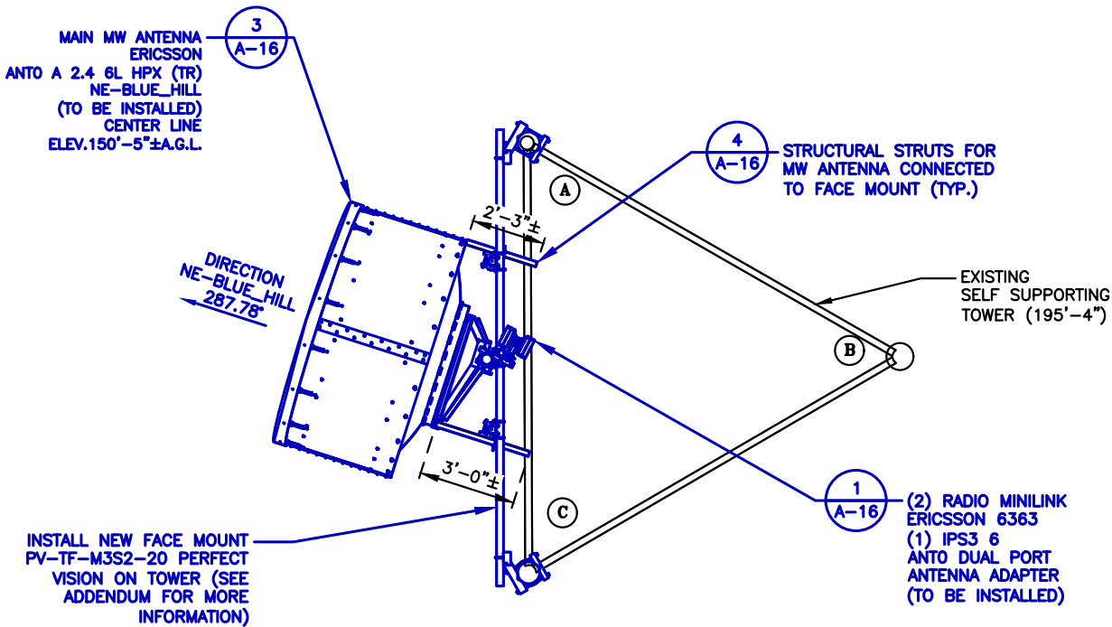
PROPOSED MW ANTENNA PLAN
