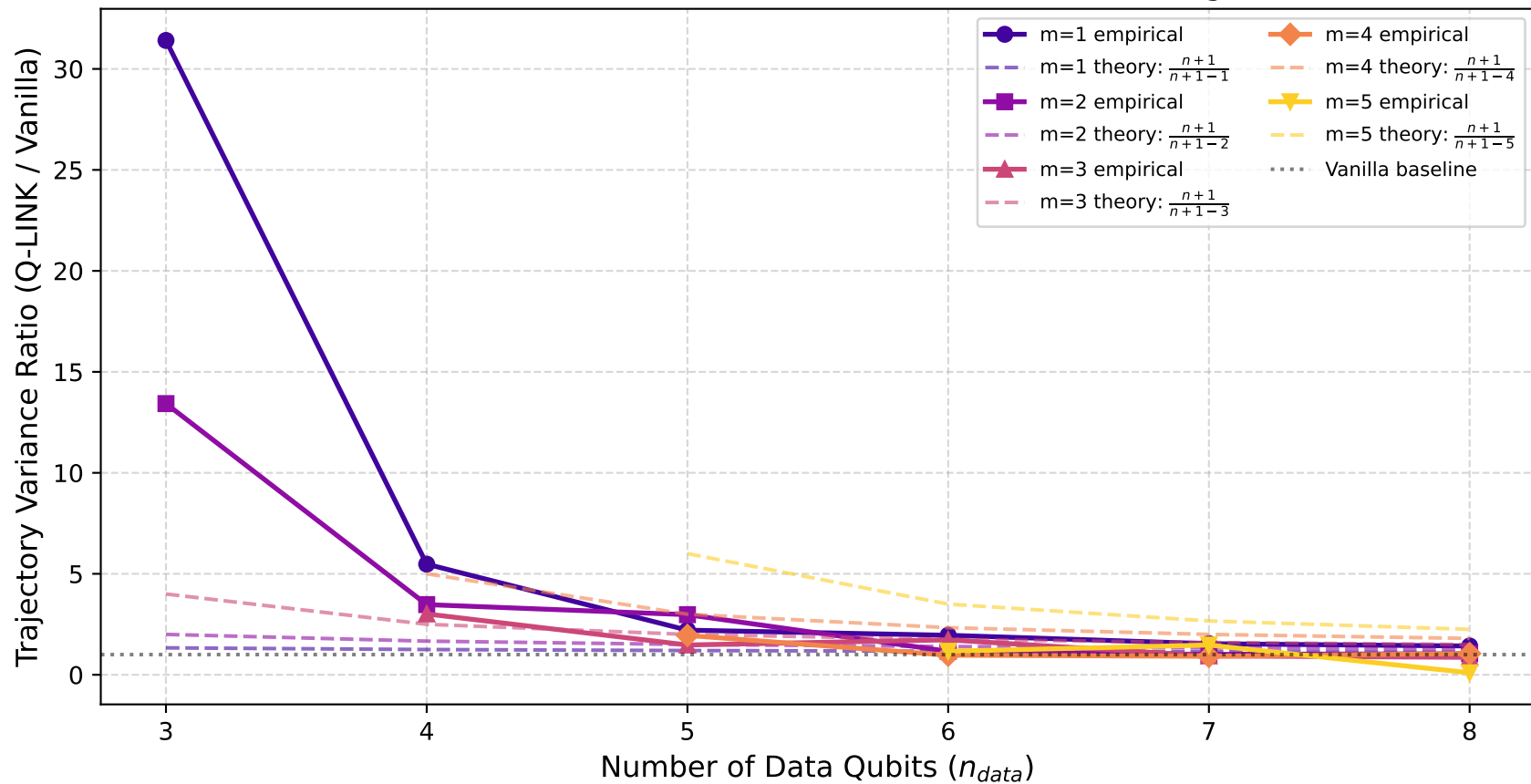
E5: m-Local Observable Combinatorial Cost Scaling
