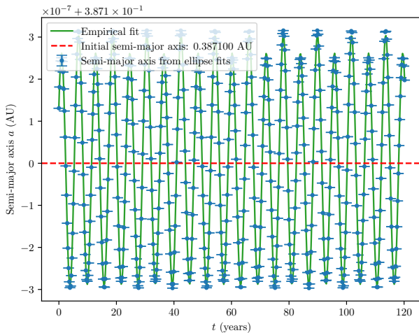
Fig. 3. Evolution of Mercury's orbital semi-major axis due to Jupiter's perturbation. The green curve is an empirical fit to equation (?). The dashed red line marks the unperturbed semi-major axis a_0 = 0.3871 AU. Unlike the eccentricity, the semi-major axis oscillates symmetrically around its initial value.
