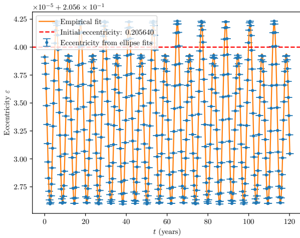
Fig. 2. Evolution of Mercury's orbital eccentricity due to Jupiter's perturbation. The orange curve is an empirical fit to equation (?). The dashed red line marks the unperturbed eccentricity \varepsilon_0 = 0.20564 . The data oscillate around a mean value \bar{\varepsilon} = 0.20563339 , systematically lower than \varepsilon_0 (see section ??).
