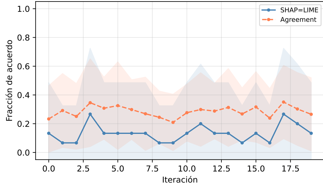
wine
