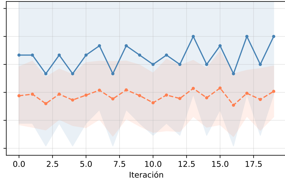
covertypes
