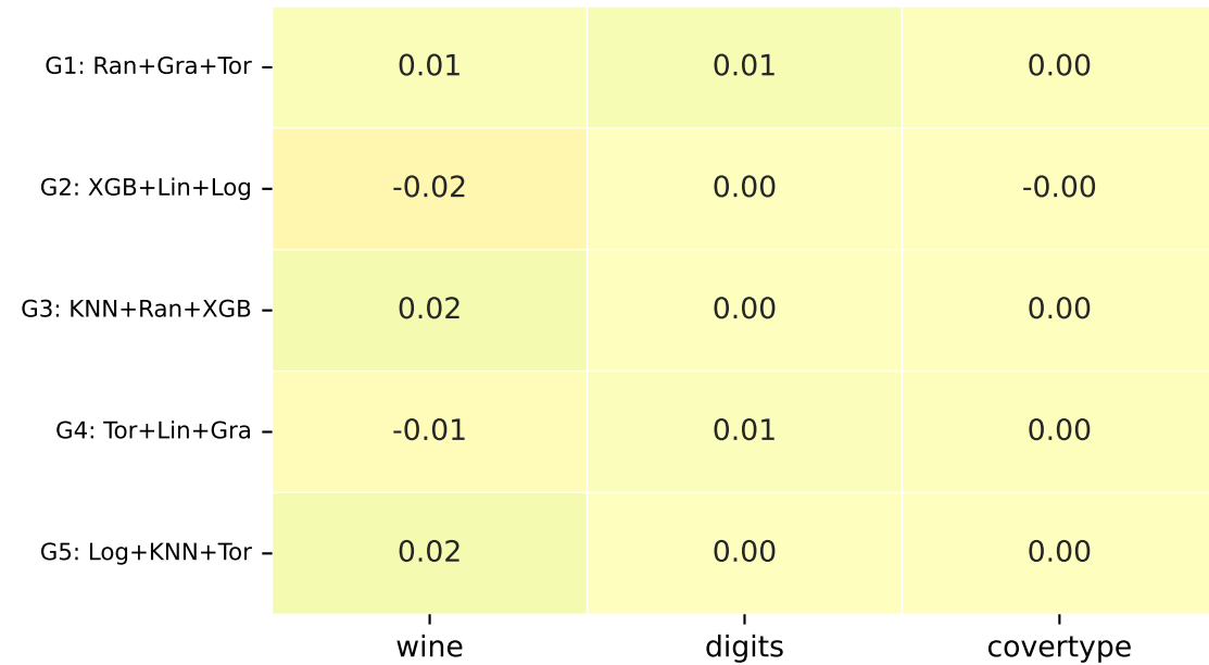
\Delta Accuracy
