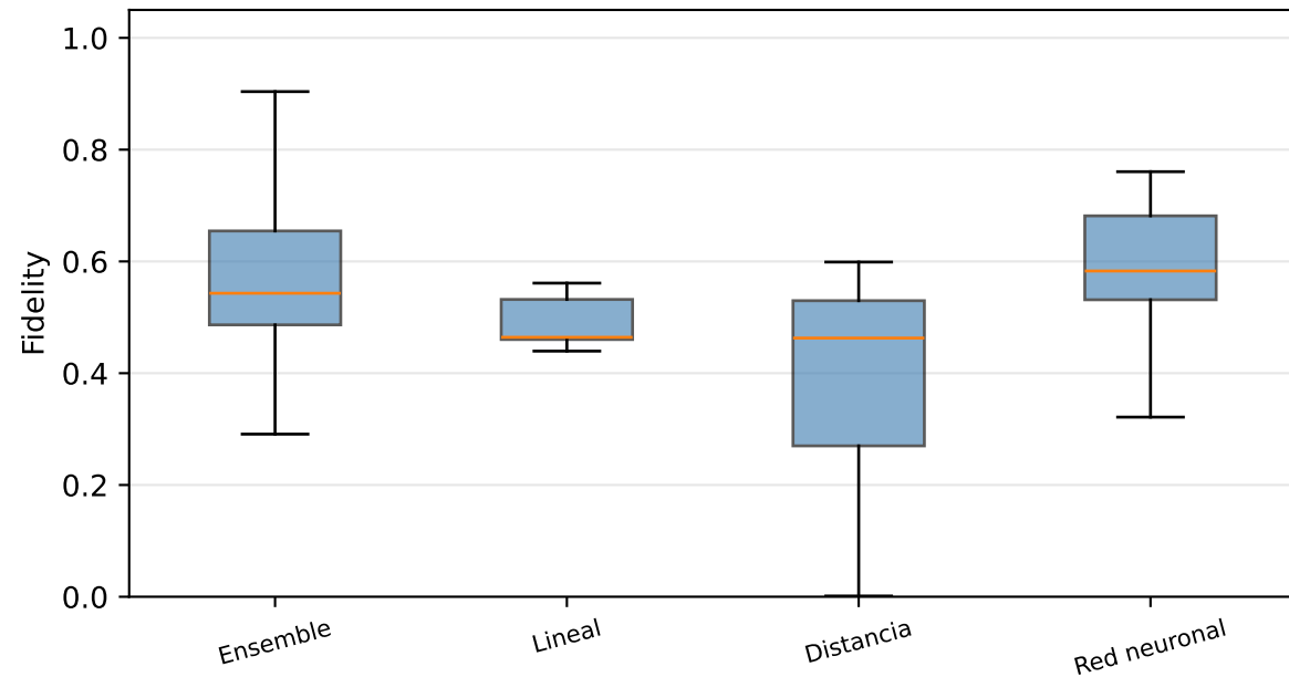
Fidelity SHAP
