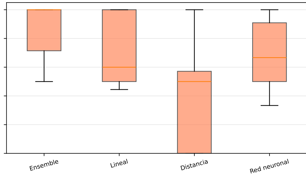
Fidelity LIME
