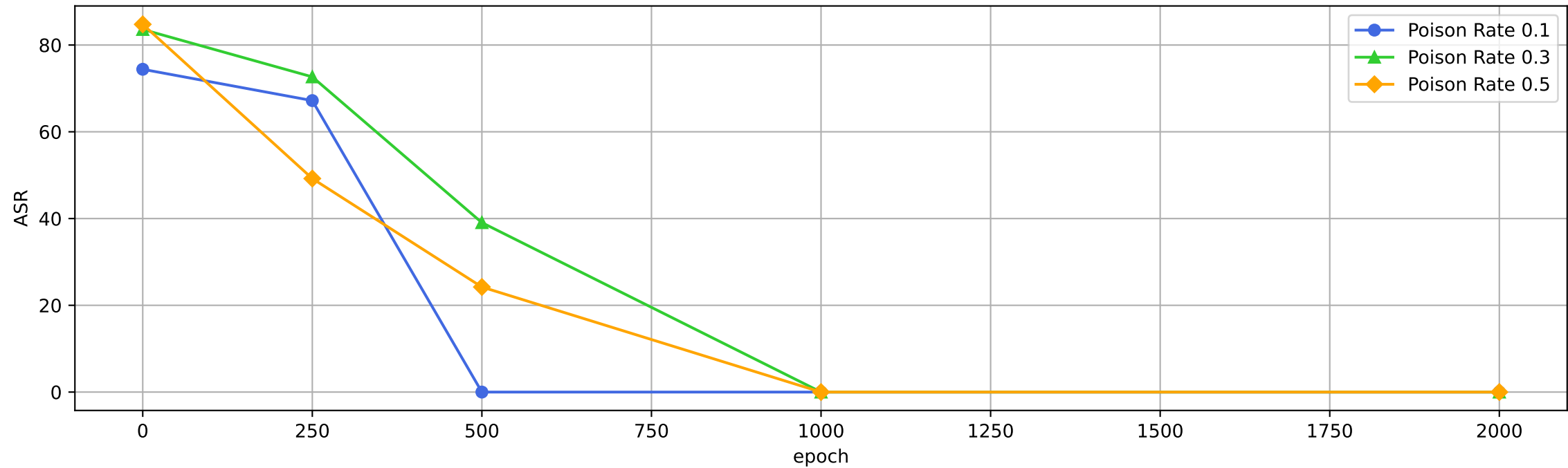
ASR of ANP v.s. train epoch
