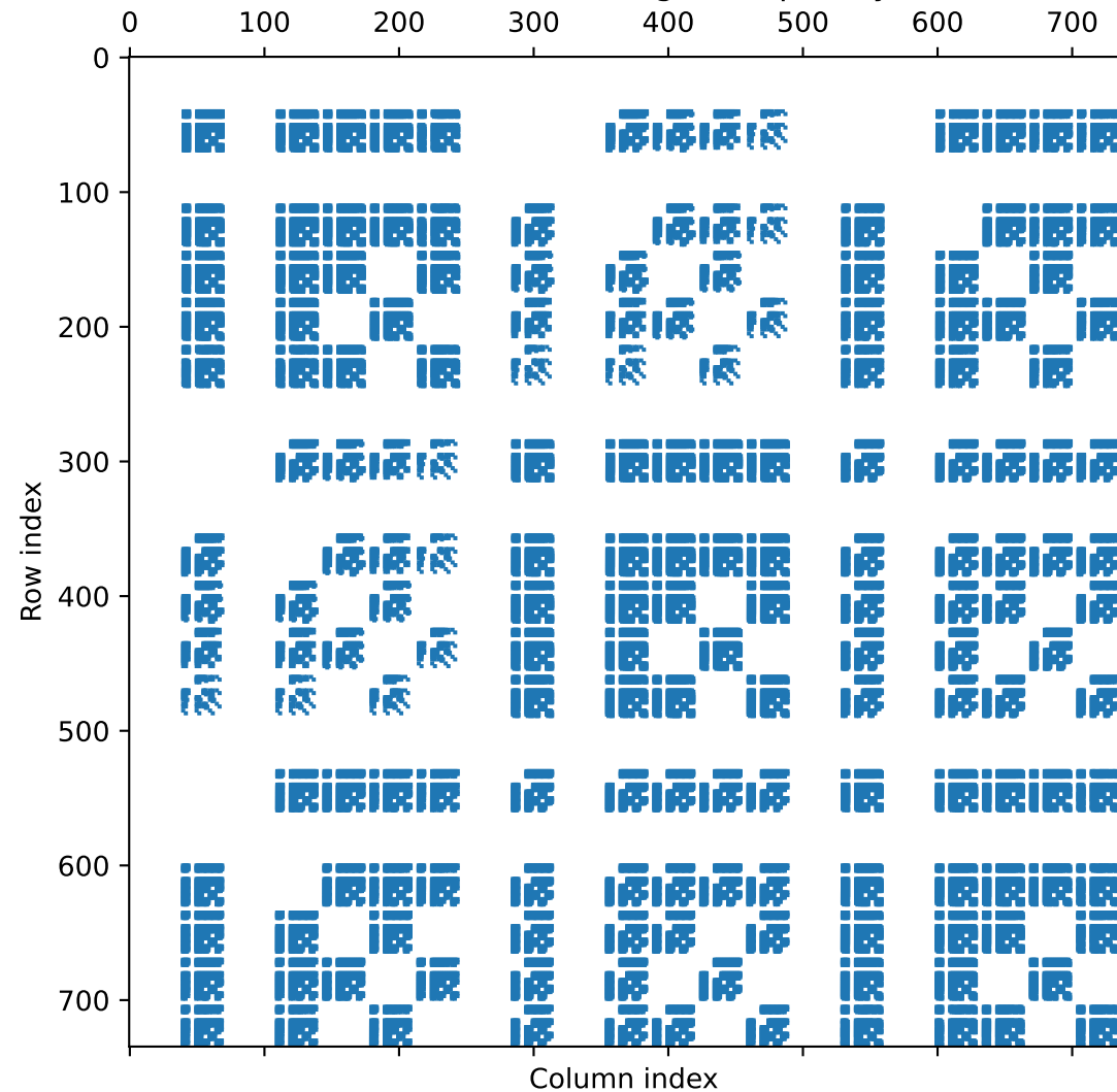
Block DOF ordering — K sparsity
