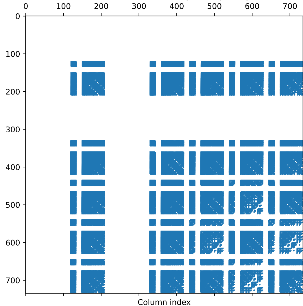
Alternated DOF ordering — K sparsity
