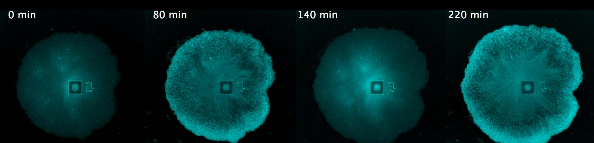
Hyperpolarised waves propagating in B. subtilis biofilm
