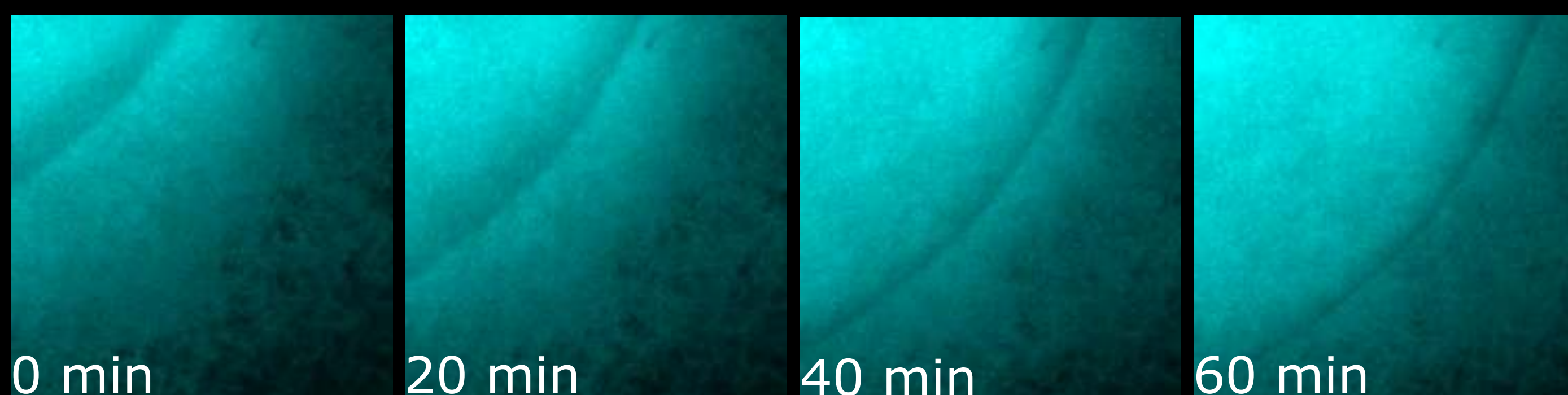
Depolarised waves propagating in B. subtilis biofilm
