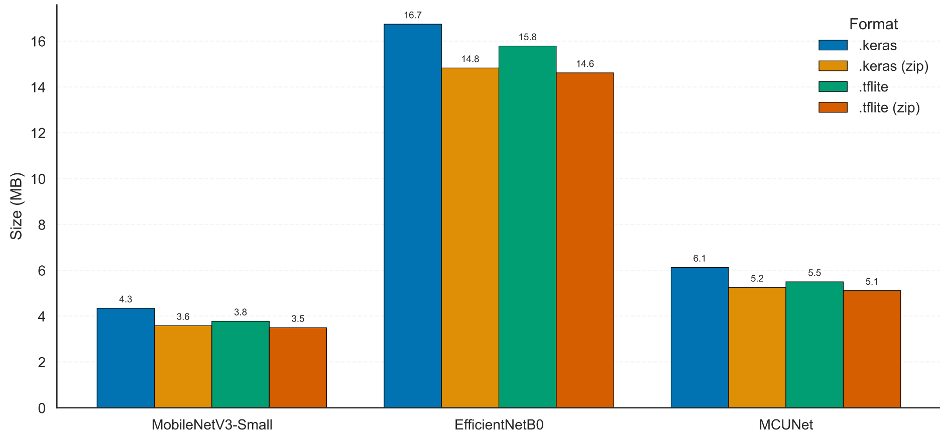
CIFAR-100: Model size comparison
