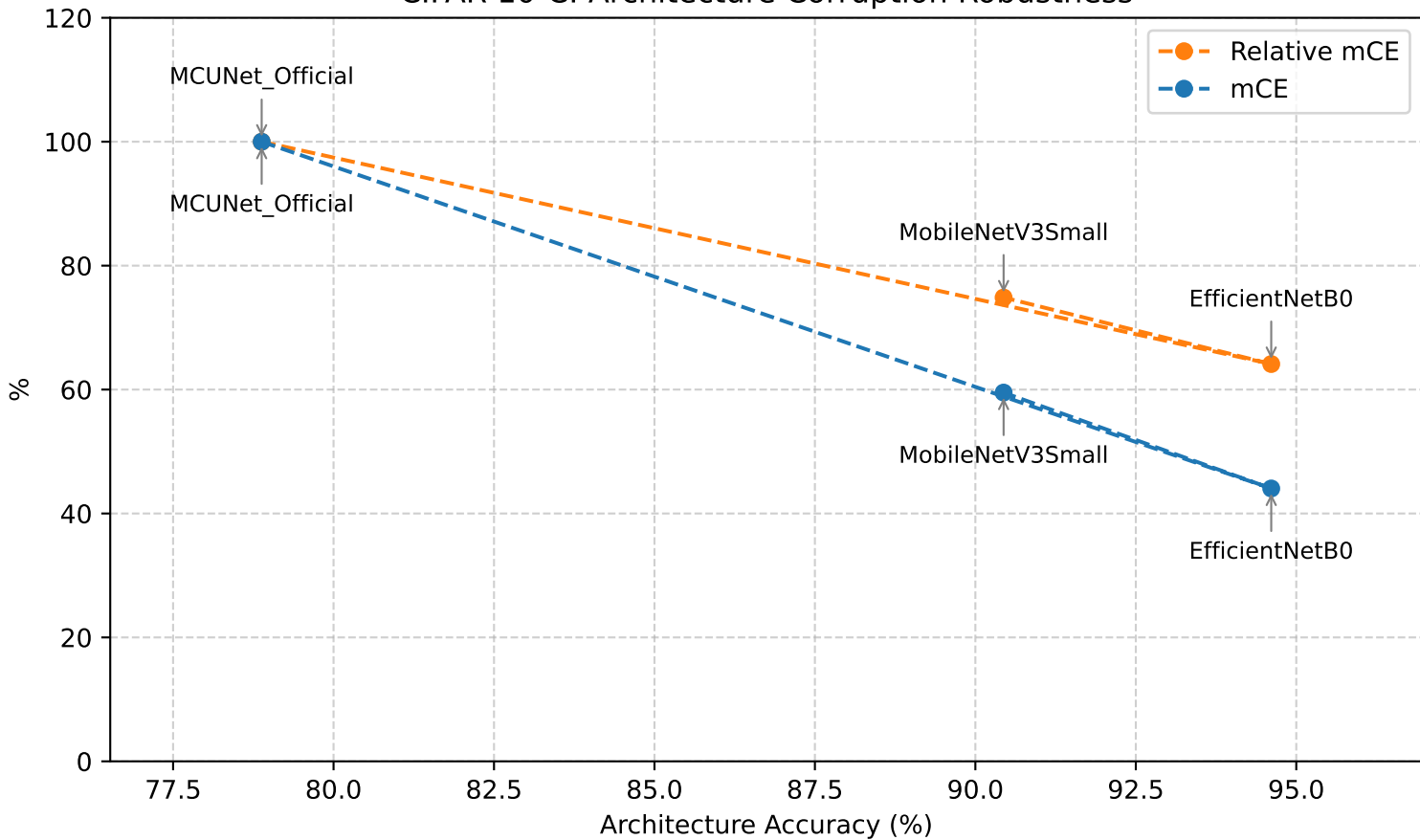
CIFAR-10-C: Architecture Corruption Robustness
