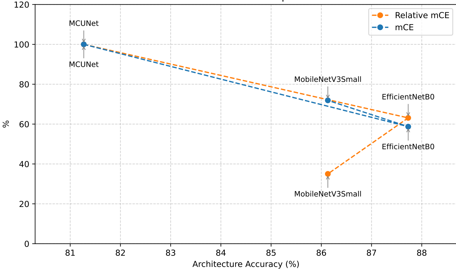
Wake Vision: Architecture Corruption Robustness
