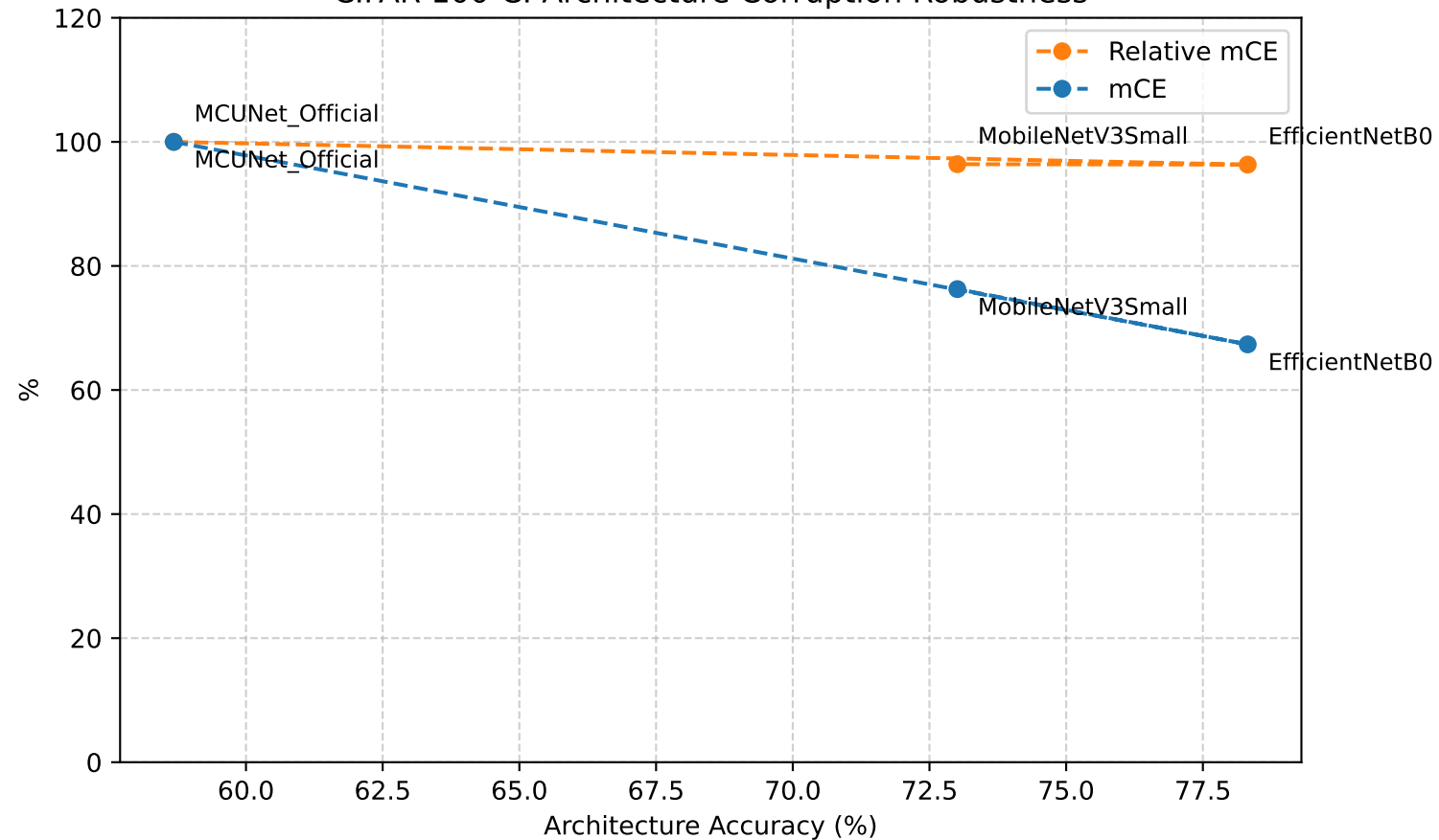
CIFAR-100-C: Architecture Corruption Robustness
