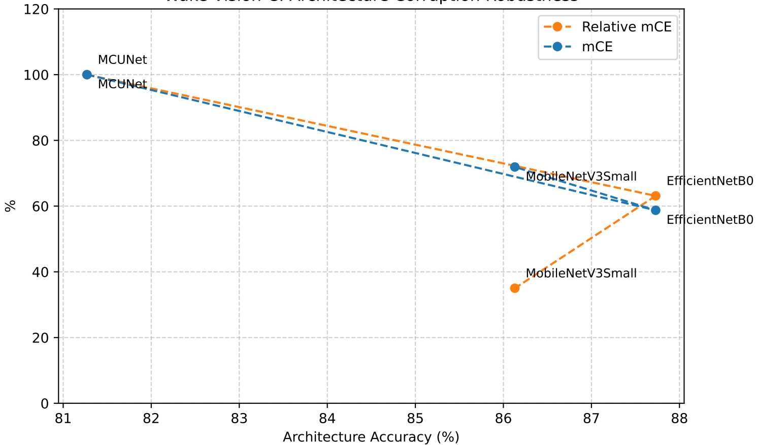
Wake Vision-C: Architecture Corruption Robustness
