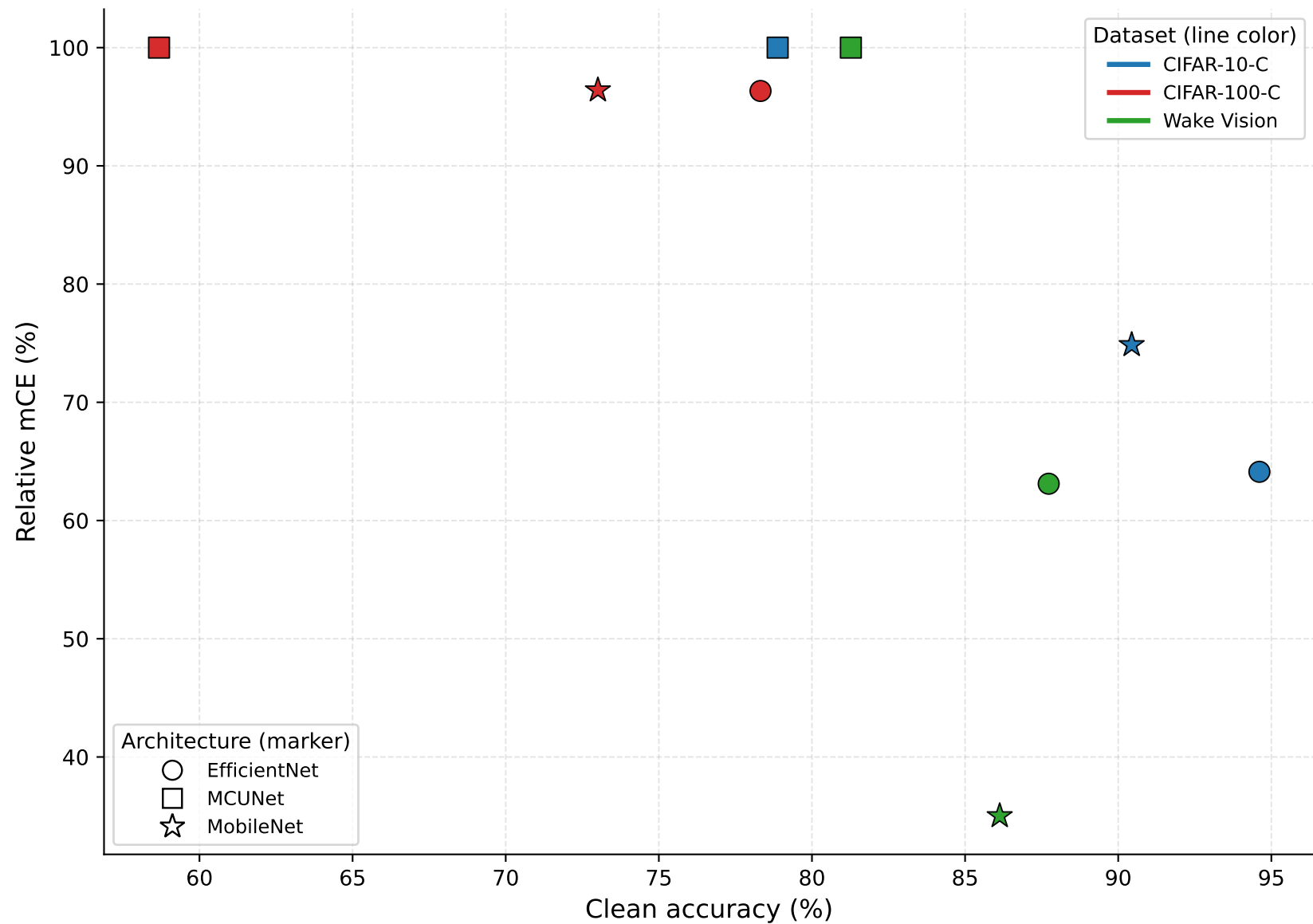
Architecture robustness across datasets
