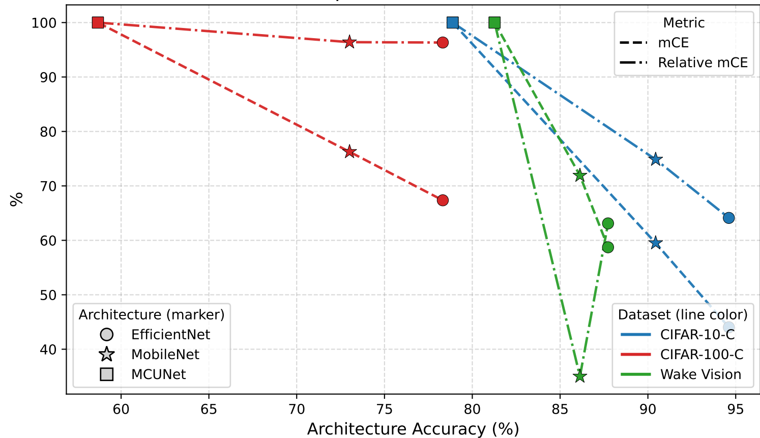
Architecture Corruption Robustness Across Datasets
