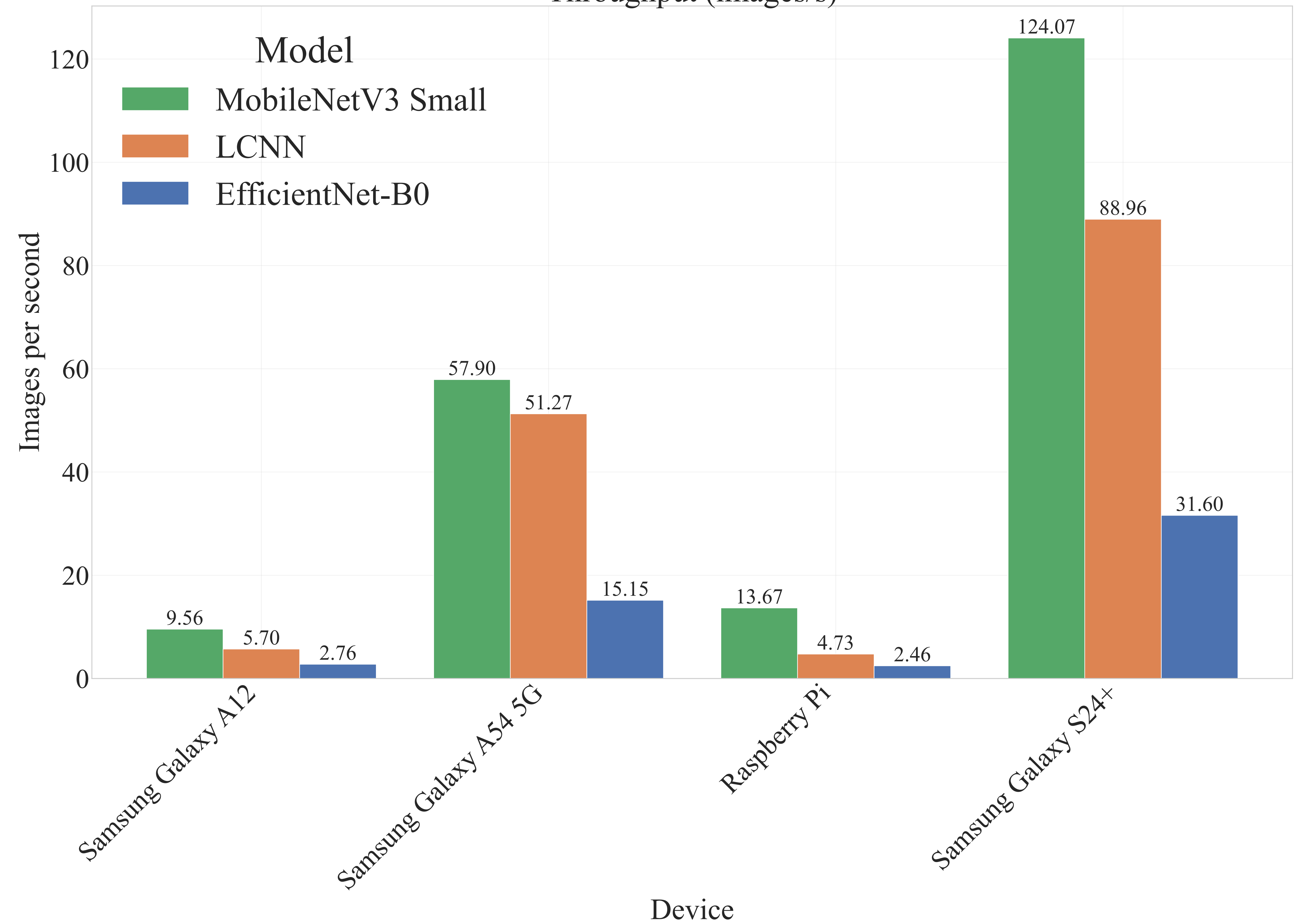
Throughput (images/s)
