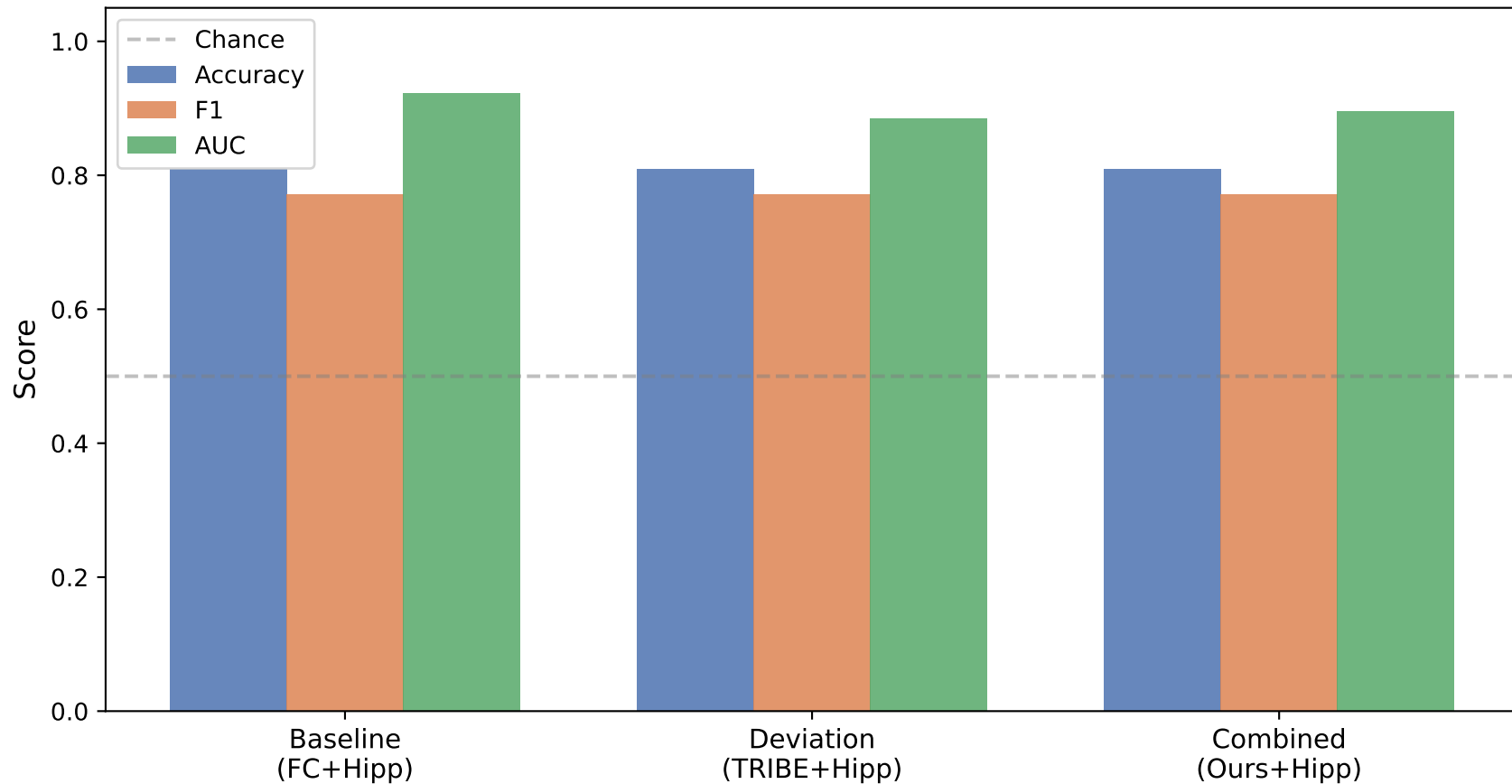
HC vs AD Classification (RF, 5-fold CV)
