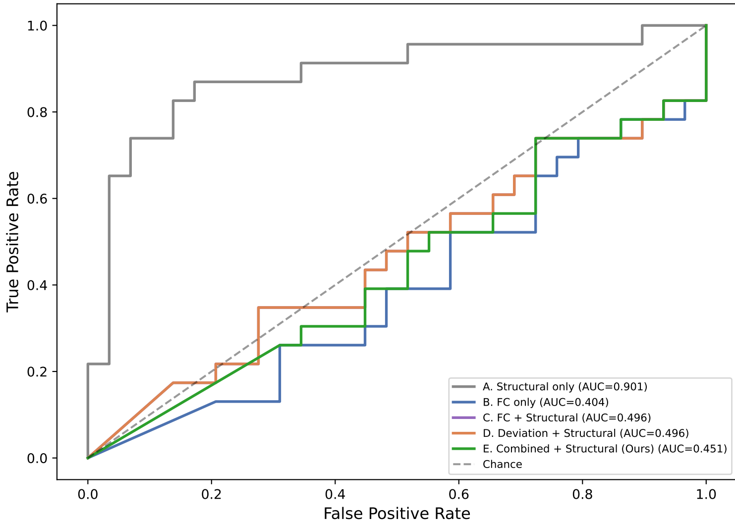
Ablation Study ROC Curves — HC vs AD (LDA)
