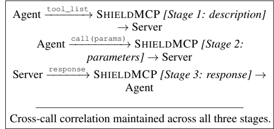
Figure 1: SHIELDMCP interposes on the JSON-RPC stream as a transparent proxy, validating tool descriptions before planning, outbound parameters before they leave the client, and inbound responses before the agent reads them.
