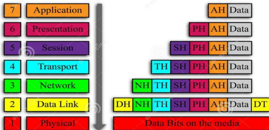
OSI Model
