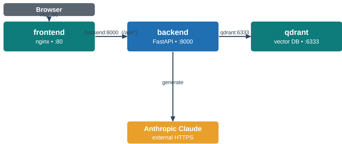
Figure 2: Inter-container communication and the port each service exposes.
