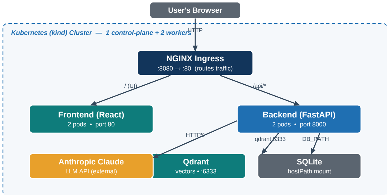
Figure 1: 3-tier architecture inside the Kubernetes cluster.
