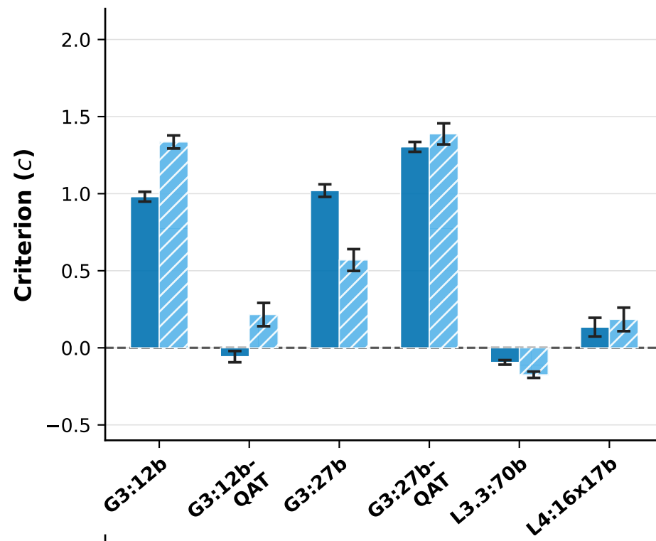
Criterion ( c )
