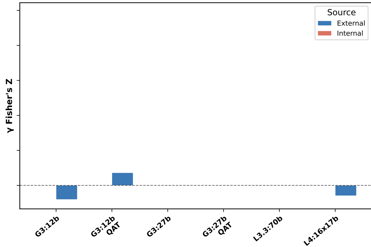
TrialChain
