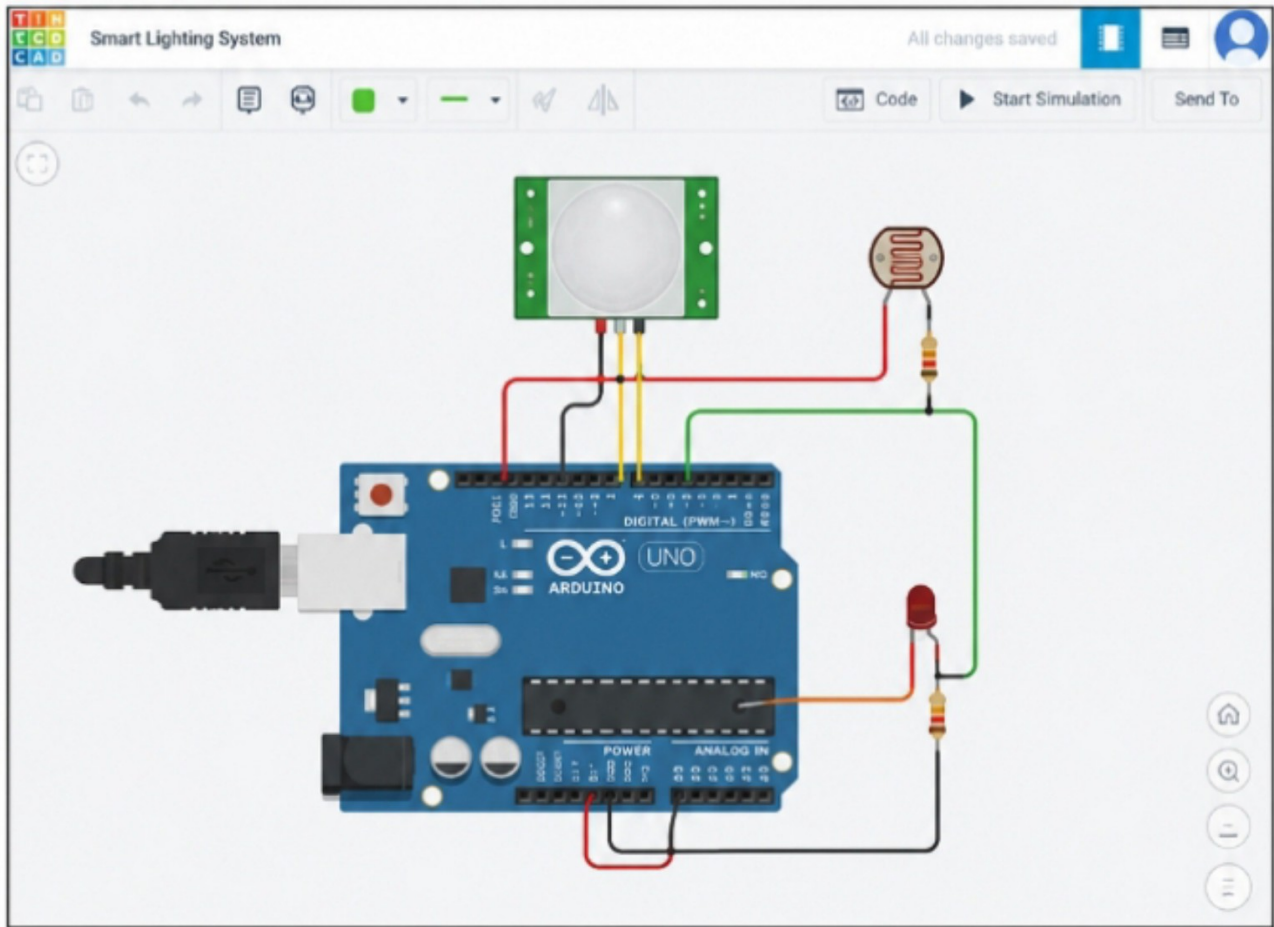
Figure 1. Tinkercad circuit simulation screenshot of the Smart Lighting System.
