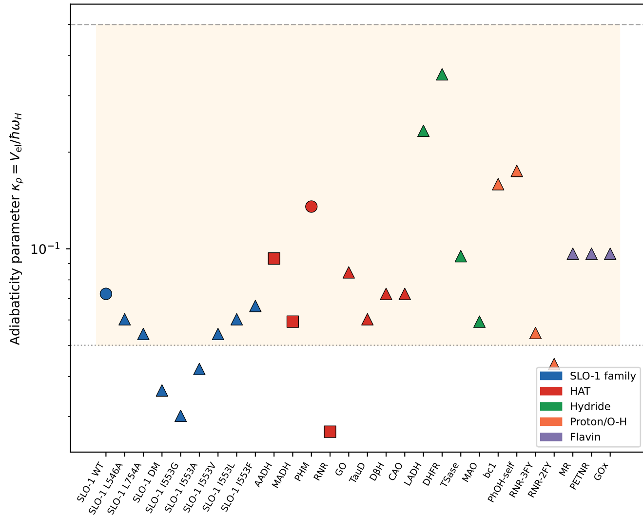
Proton-transfer adiabaticity across 28 systems
