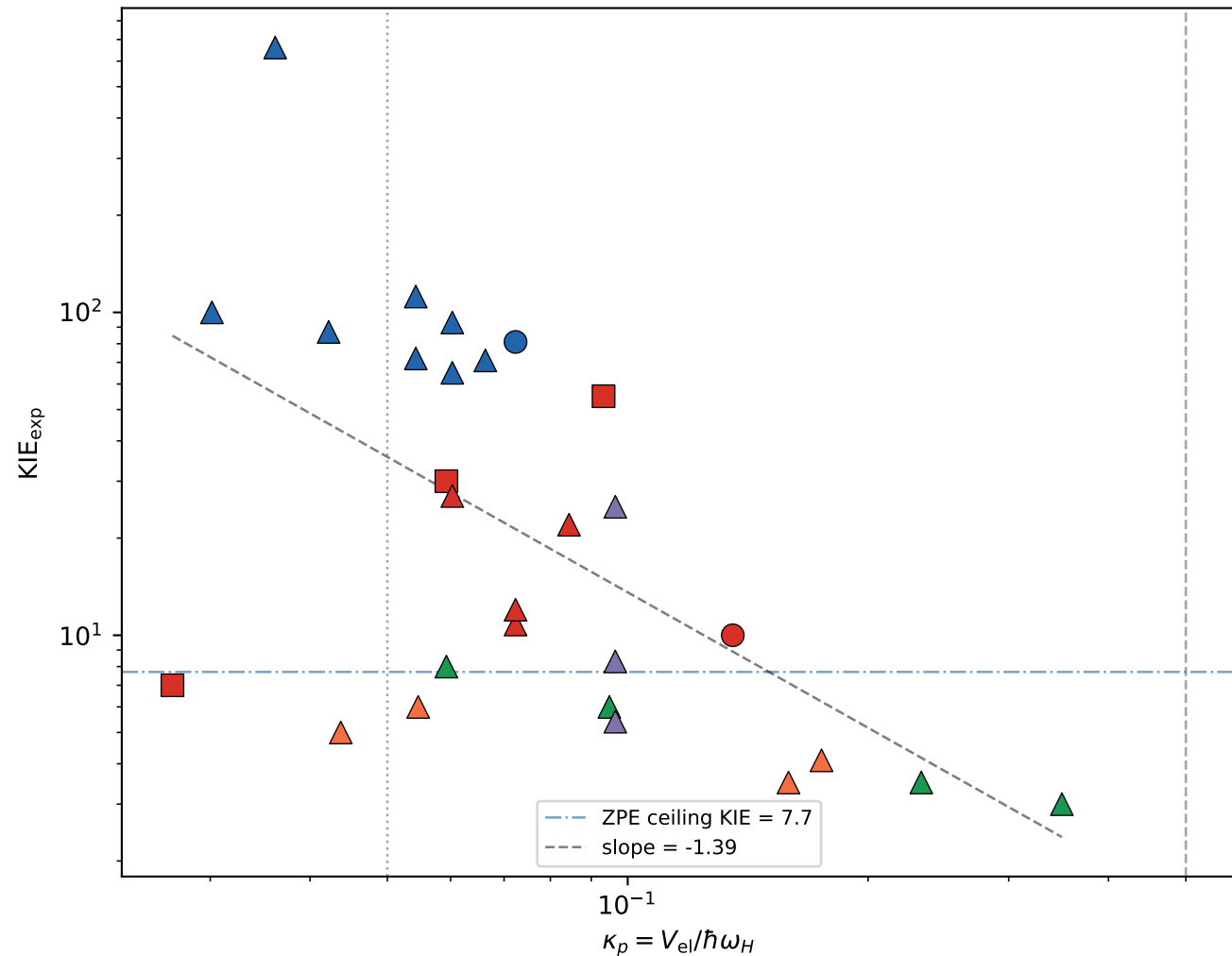
KIE vs adiabaticity ( r = -0.58 in log-log)
