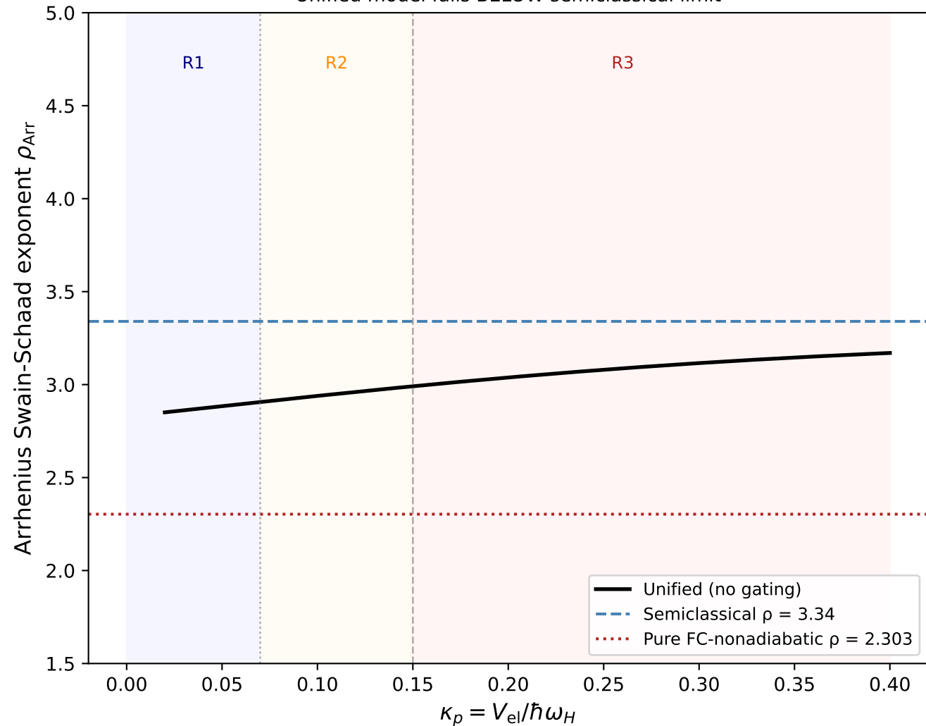
Analytical \rho_{\text{Arr}} vs \kappa_p (no gating) Unified model falls BELOW semiclassical limit
