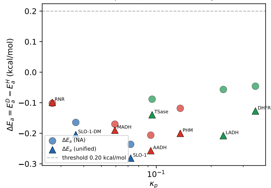
Isotope \Delta E_a vs adiabaticity
