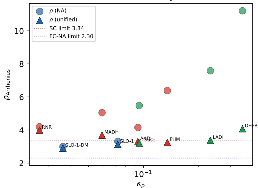
Arrhenius Swain-Schaad exponent vs adiabaticity
