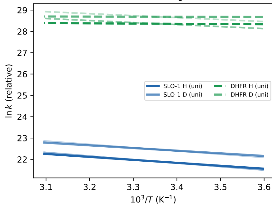
Arrhenius plots: SLO-1 vs DHFR (solid=H, dashed lighter=D)
