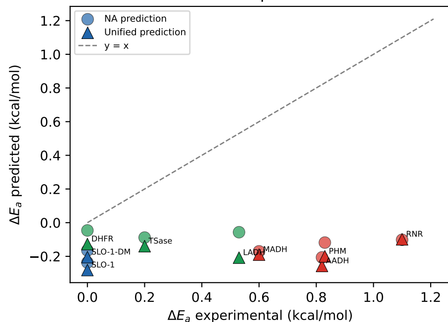
Predicted vs experimental \Delta E_a
