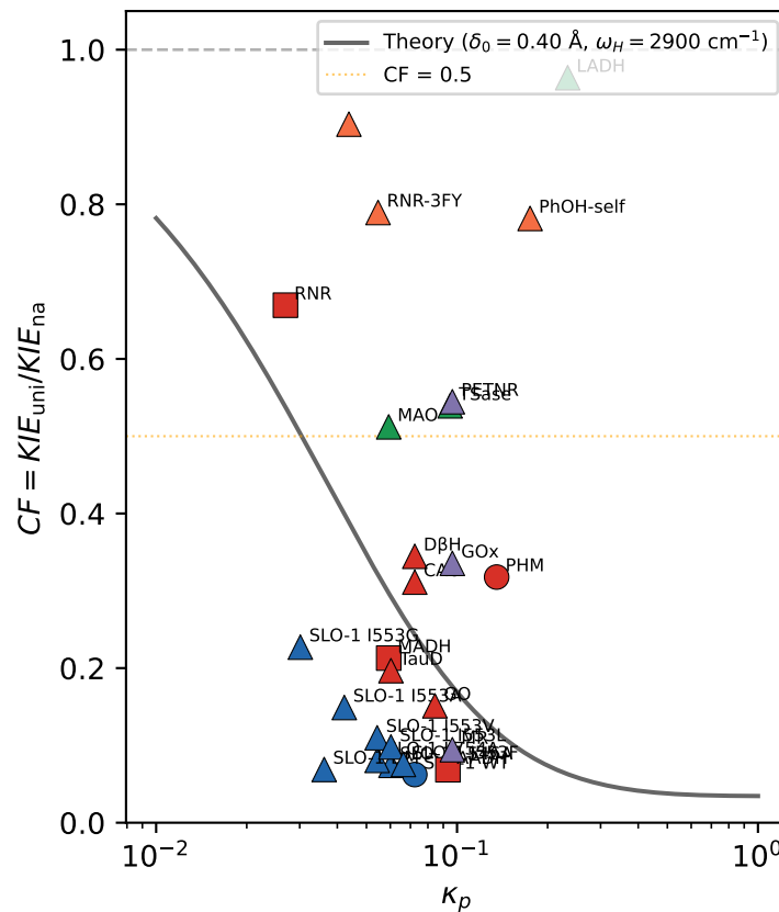
Adiabatic correction to KIE
