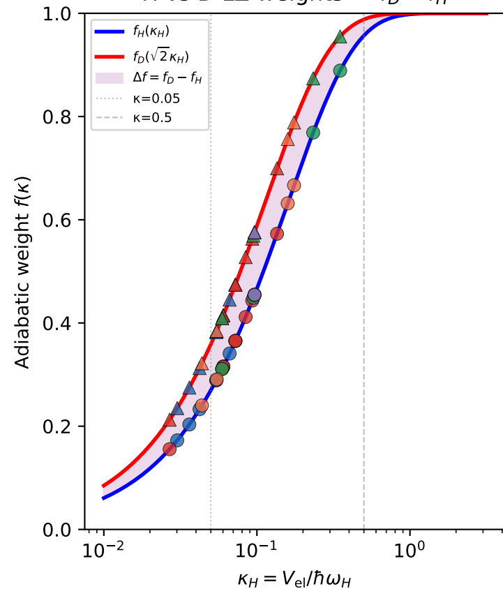
H vs D LZ weights — f_D > f_H
