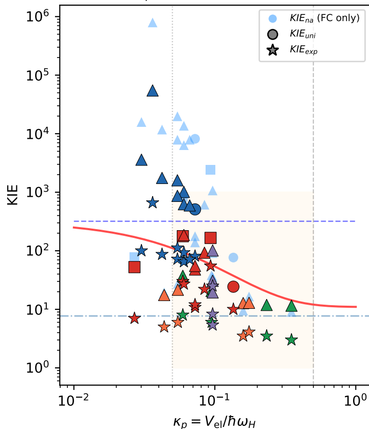
KIE vs \kappa_p — NA, unified, and exp
