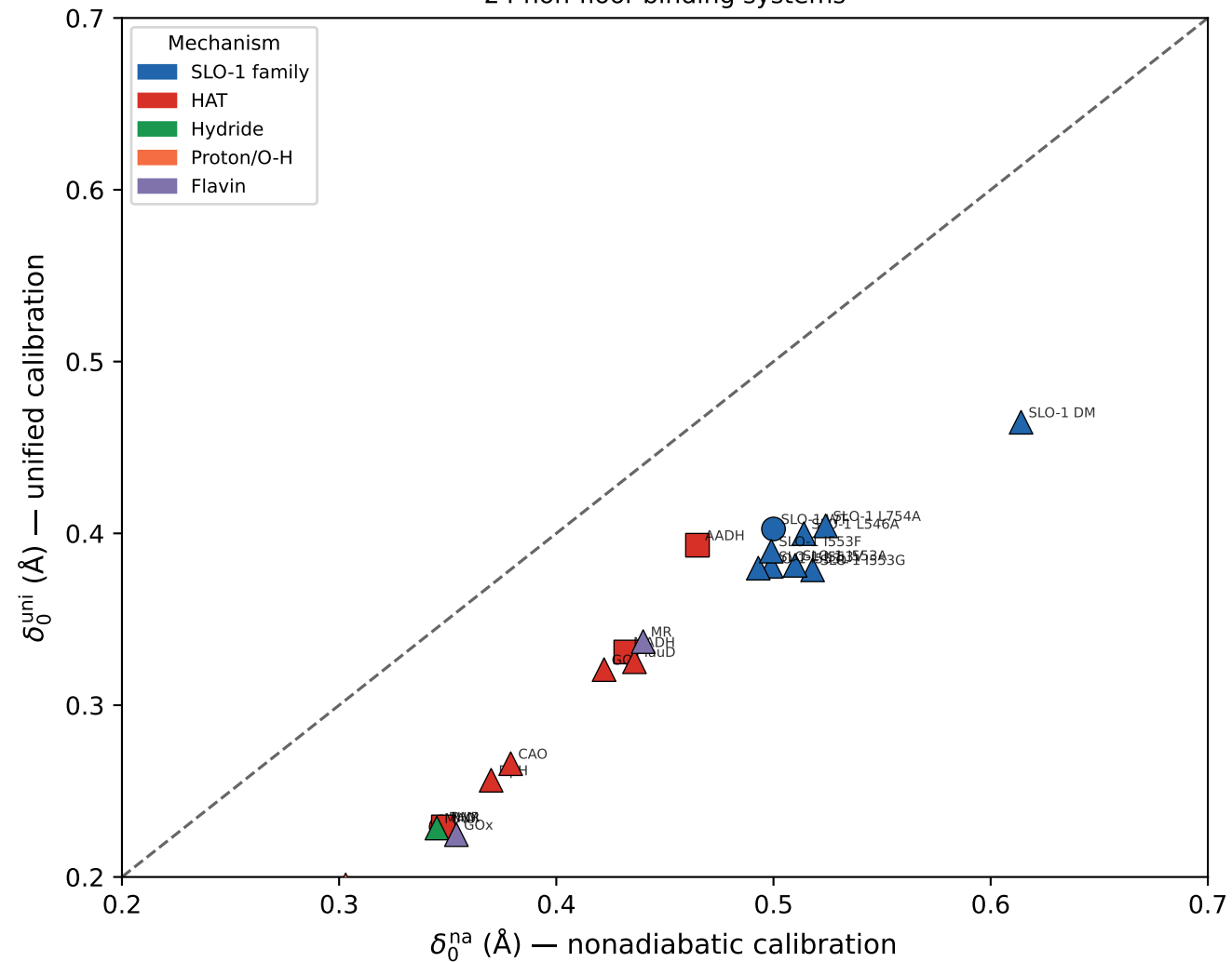
Self-consistent recalibration ( r = 0.980 ) 24 non-floor-binding systems
