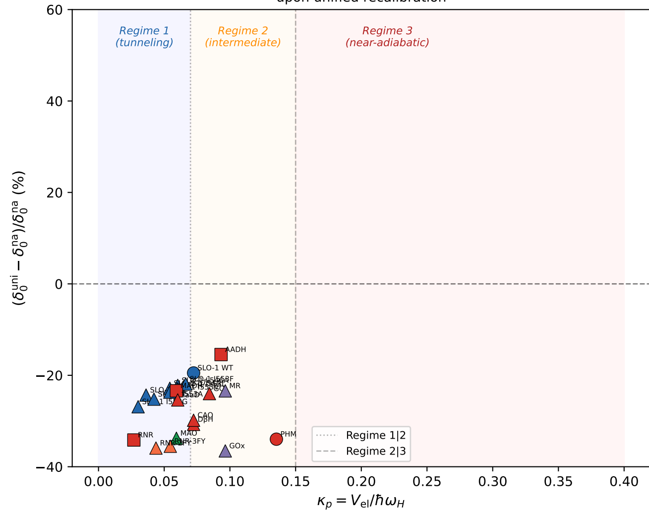
Fractional shift in donor-acceptor geometry upon unified recalibration
