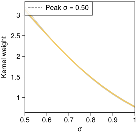
a Learned RH kernel (NN-GAUSS)
