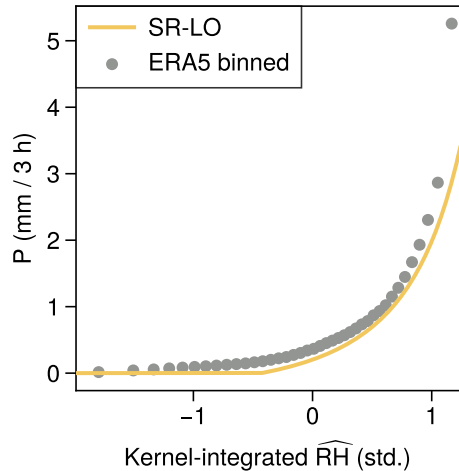
c ERA5 observed vs SR-LO
