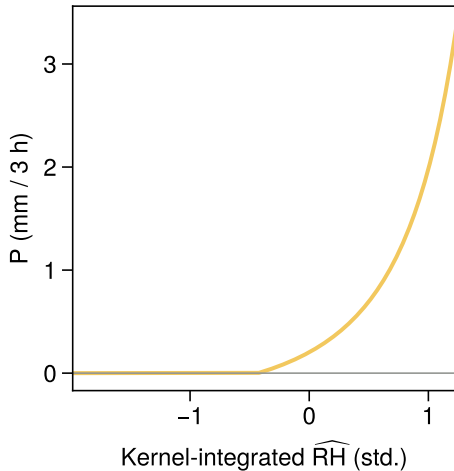
b SR-LO: P vs kernel-integrated RH
