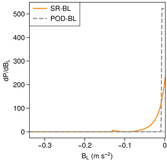
b Precipitation sensitivity dP/dB_L
