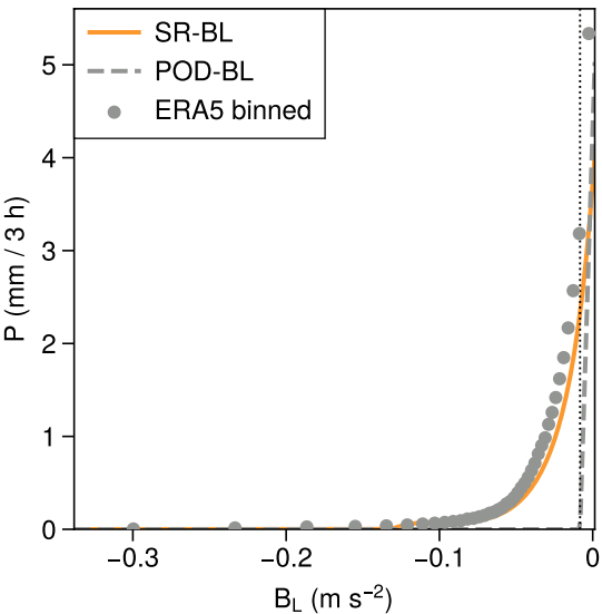
a Mean P vs B_L : ERA5 and learned models
